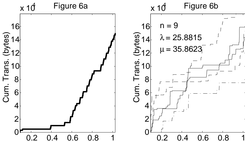
FIGURE 6: Another estimation - simulation example showing that while our model gives the right number and size of flat spots, it does not effectively model TCP slow start.
