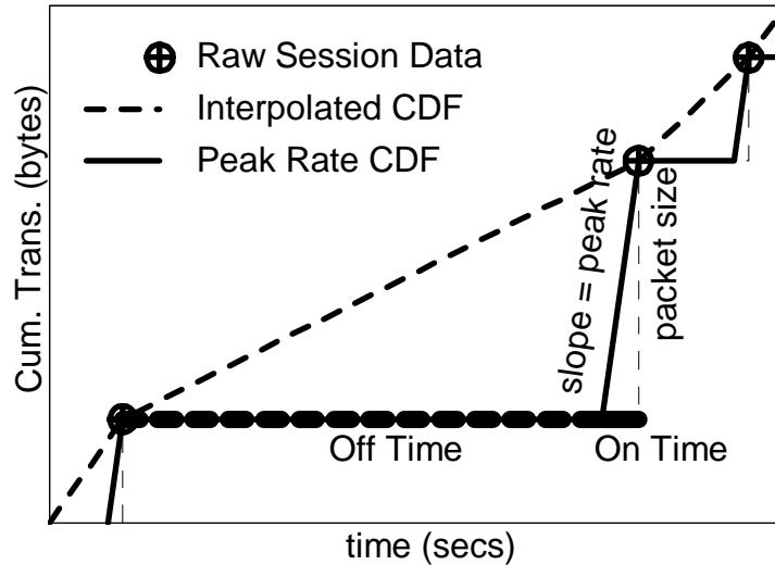
FIGURE 3: Zoomed in plot of a TCP connection trace, showing raw data, and how the peak rate is used to determine on and off times.
