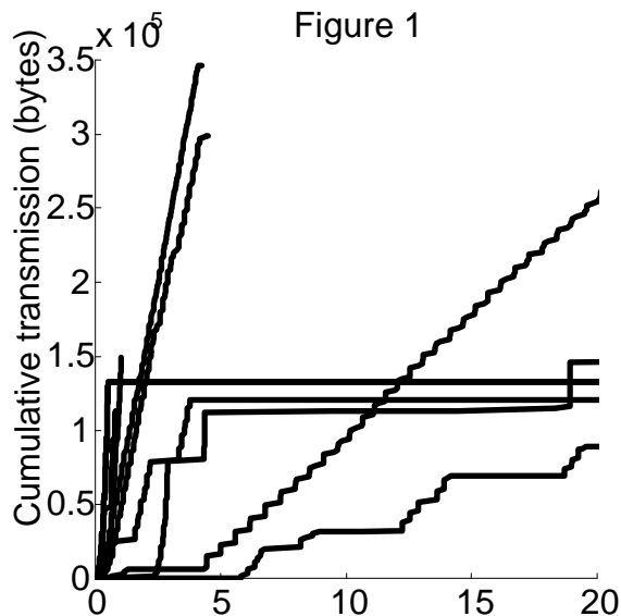
FIGURE 1: TCP connection traces (some only partial for easy comparison), showing cumulative transmission as a function of time. This illustrates the diversity of this population.
