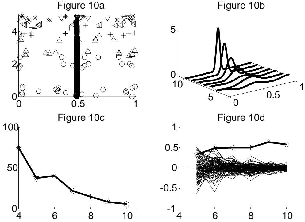
FIGURE 10: Statistical analyses of decomposed conservative cascade generators for trace of Figure 4a. Figure 10a is an order plot of the raw generators. Figure 10b shows level wise kernel smoothed histograms. Figure 10c show the levelwise percent inside the interval [0.45, 0.55] . Figure 10d shows the correlation between level j and j - 1 .
