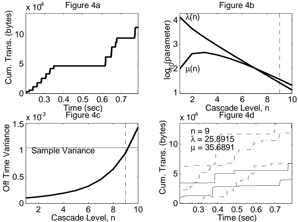
FIGURE 4: Raw data trace is in Figure 4a, with the estimation process illustrated in Figures 4b and 4c. Figure 4d shows 5 simulated traces from the model with estimated parameters, showing similar qualitative structure.
