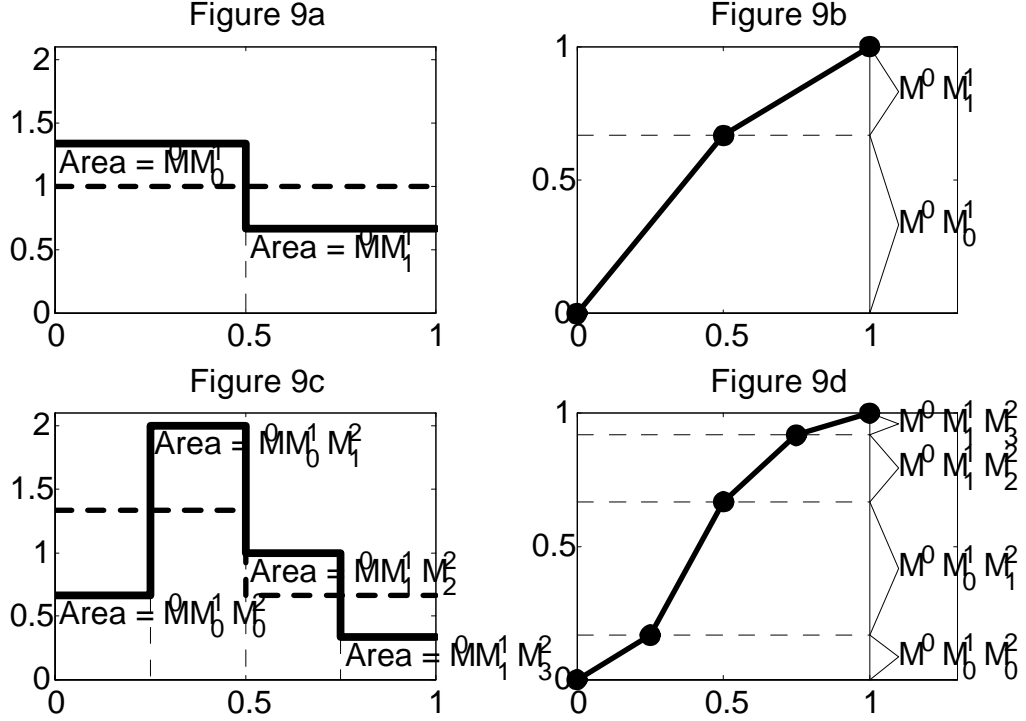
FIGURE 9: Toy example illustrating the conservative cascade construction. Figure 9a shows the rate function r_1 and Figure 9b shows the corresponding cumulative for n = 1 . Figure 9c shows the rate function r_2 and Figure 9d shows the corresponding cumulative for n = 2 .
