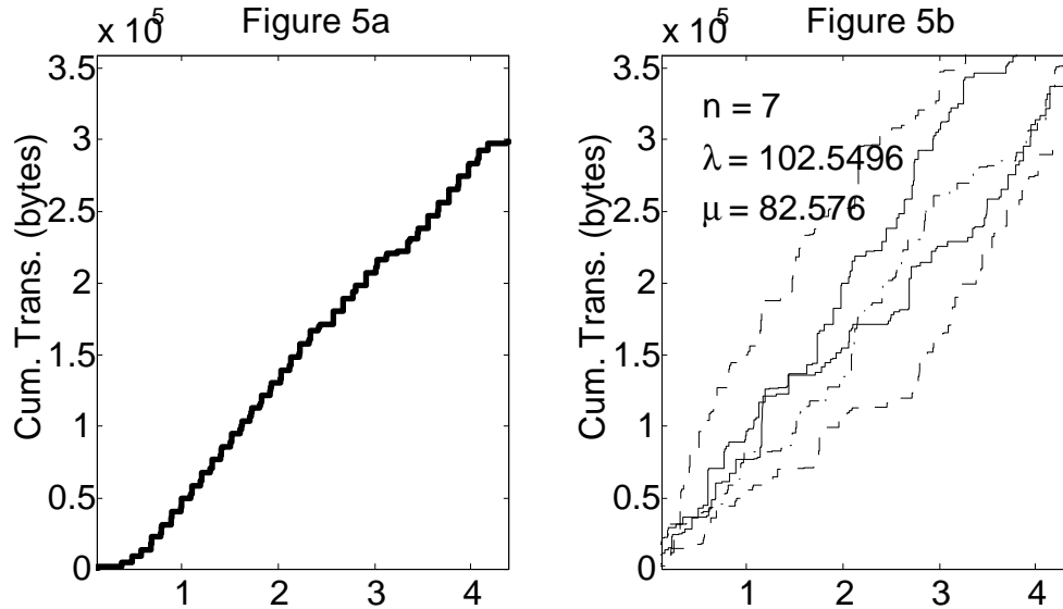
FIGURE 5: Another trace, Figure 5a, together with 5 traces simulated from the estimated model. This again shows good visual fit of the model.
