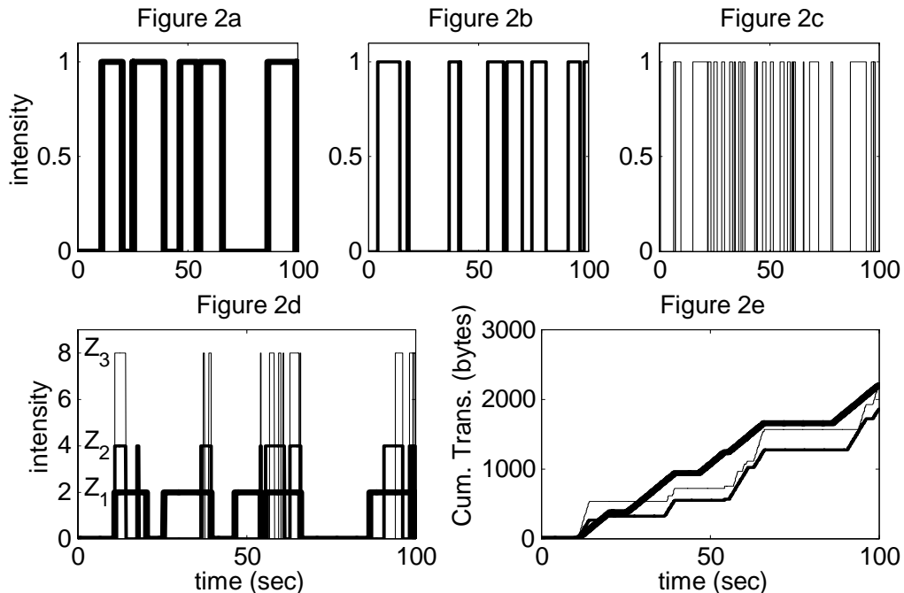
FIGURE 2: Toy Example showing how multiplying On-Off processes produces diverse off times. Figures 2a, b and c show one realization of X_1 , X_2 and X_3 respectively. Their normalized products, Z_1 , Z_2 and Z_3 are shown in Figure 2d, and the corresponding cumulatives in Figure 2e.
