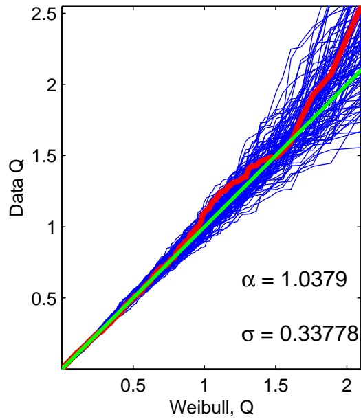
Weibull QQ Plot – On Times
