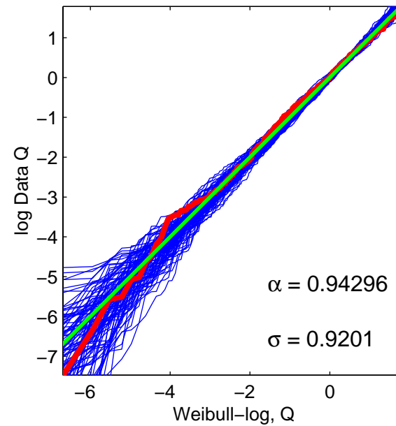
log Weibull QQ Plot – Off Times
