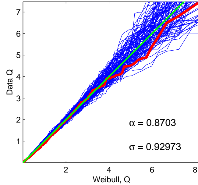
Weibull QQ Plot – Off Times
