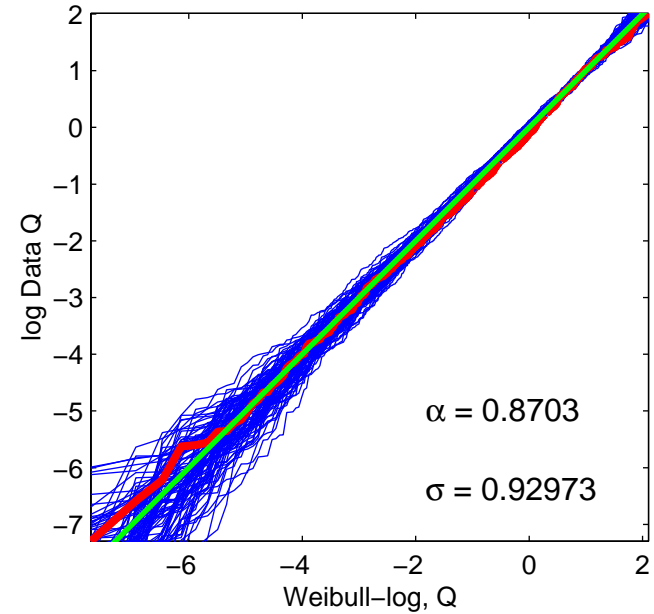
log Weibull QQ Plot – Off Times
