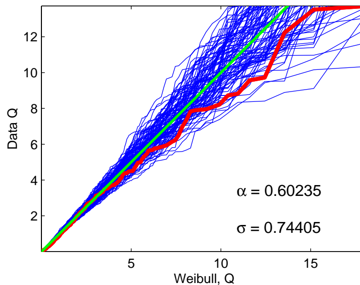
Weibull QQ Plot – Off Times
