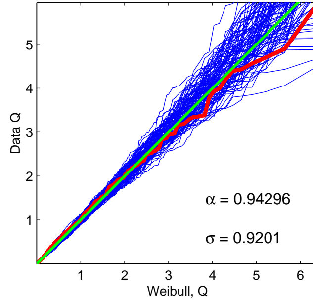
Weibull QQ Plot – Off Times
