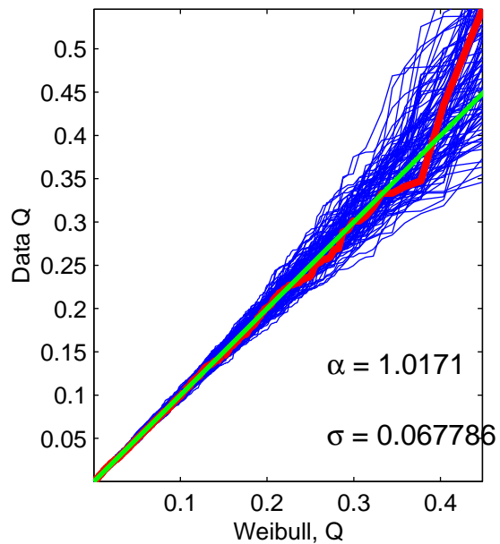
Weibull QQ Plot – On Times
