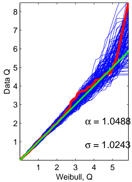
Weibull QQ Plot – On Times
