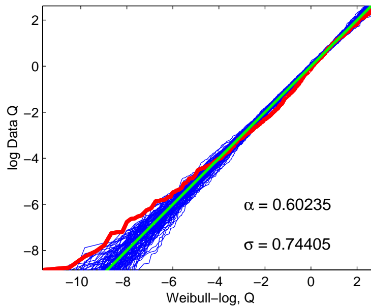
log Weibull QQ Plot – Off Times
