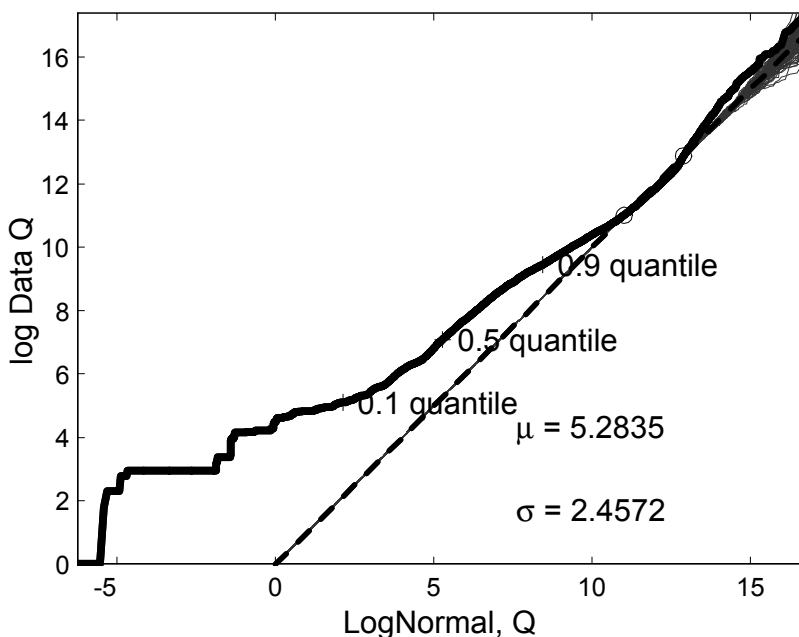
FIGURE 4: Log-normal Q-Q plot for the respnose data. Shows fit is not much worse than for the Pareto.
