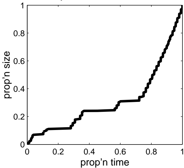
Interarrival times
