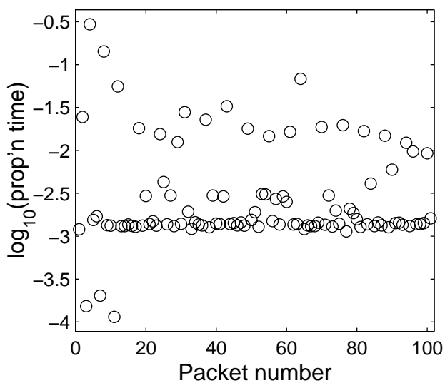
\log_{10} Interarrival times
