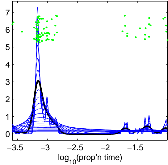
SiZer Map
