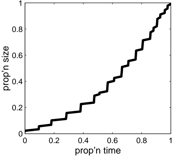
Interarrival times
