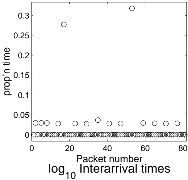
Interarrival times
