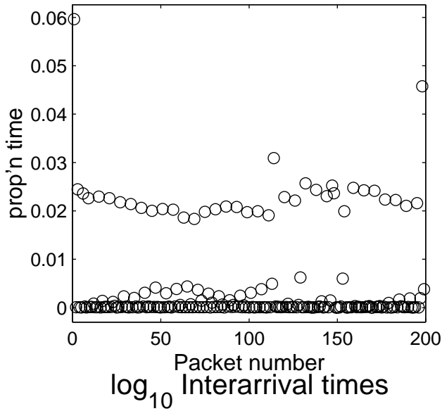
Interarrival times
