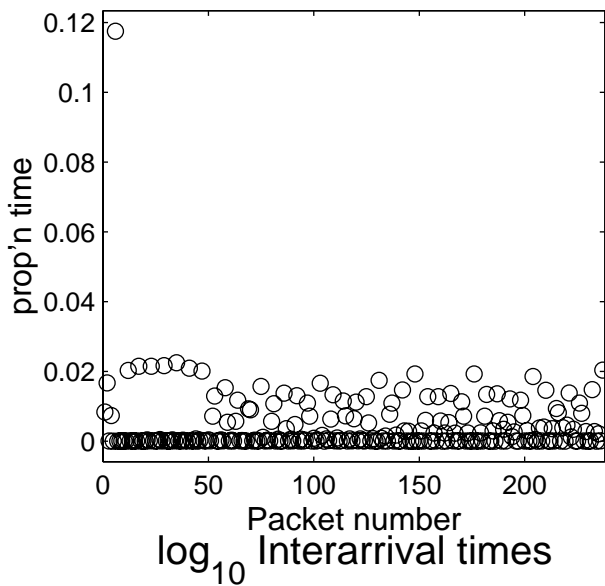
Interarrival times
