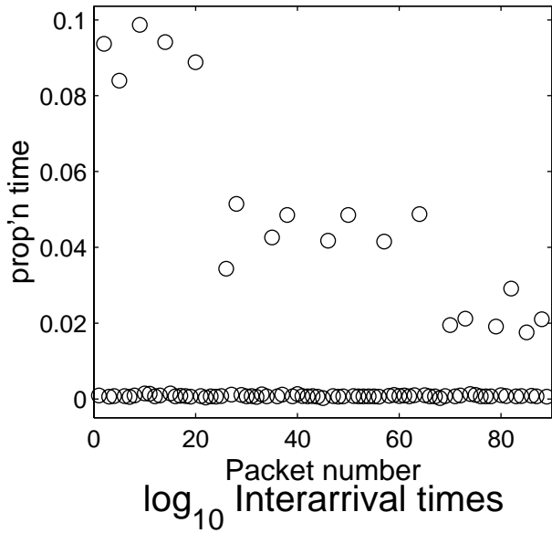
Interarrival times
