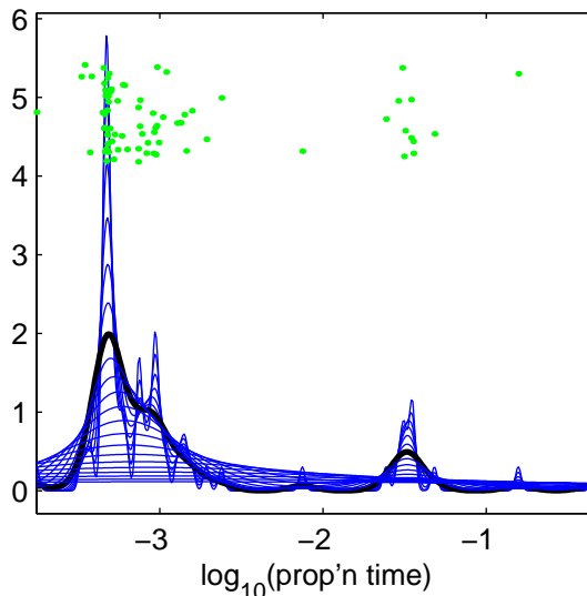
SiZer Map
