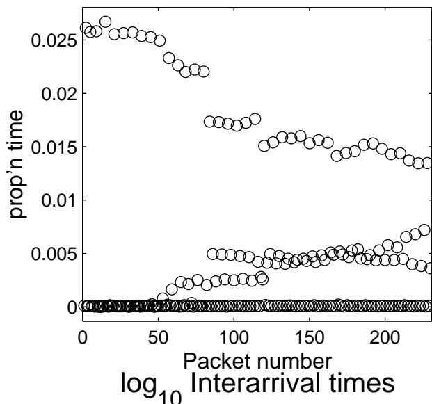
Interarrival times
