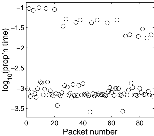
\log_{10} Interarrival times
