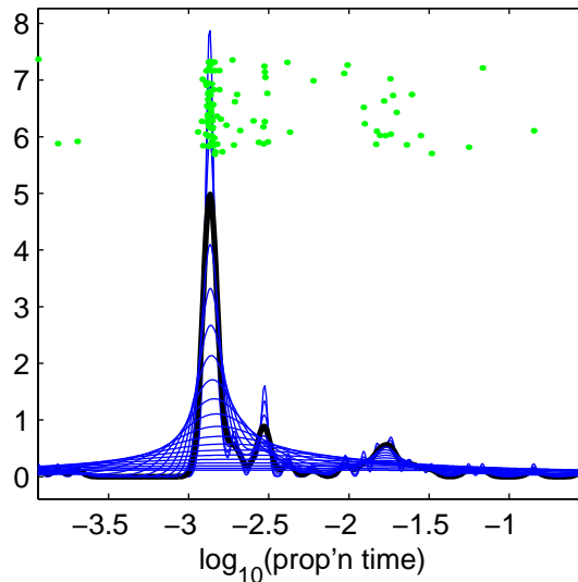
SiZer Map
