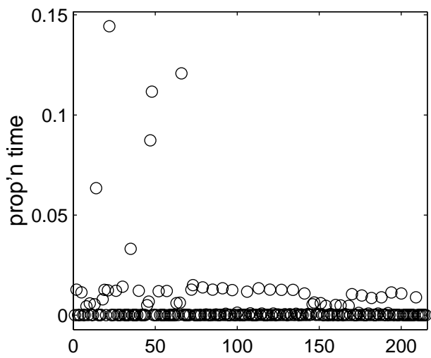
\log_{10} Interarrival times
