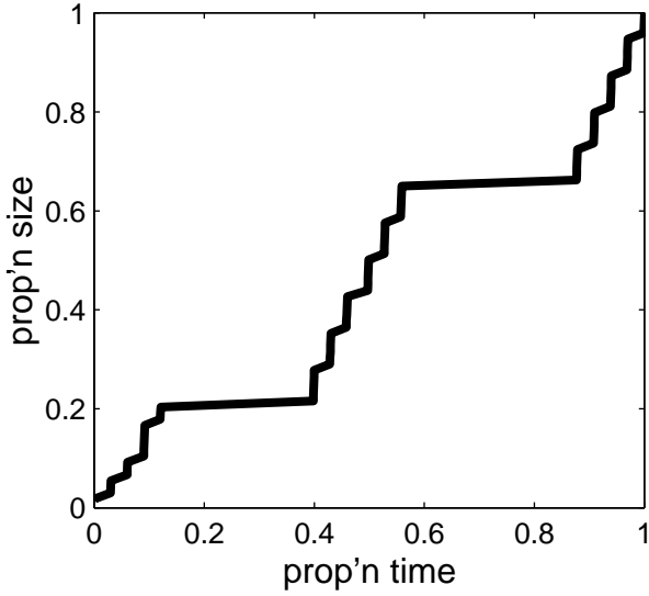
Interarrival times
