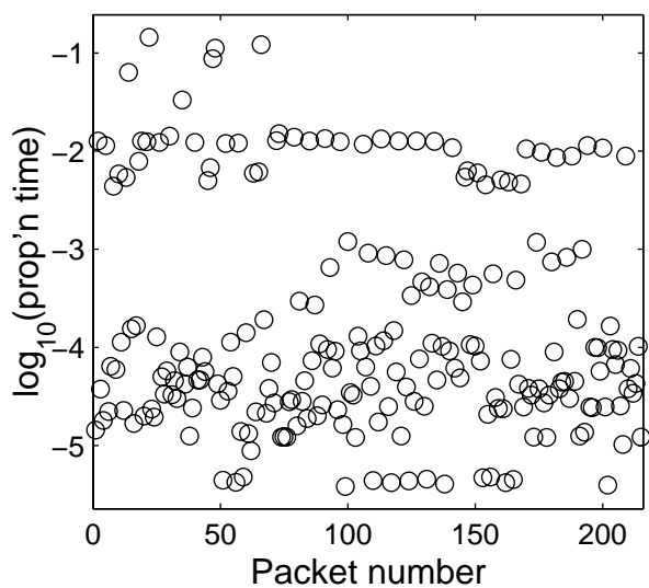
\log_{10} Interarrival times
