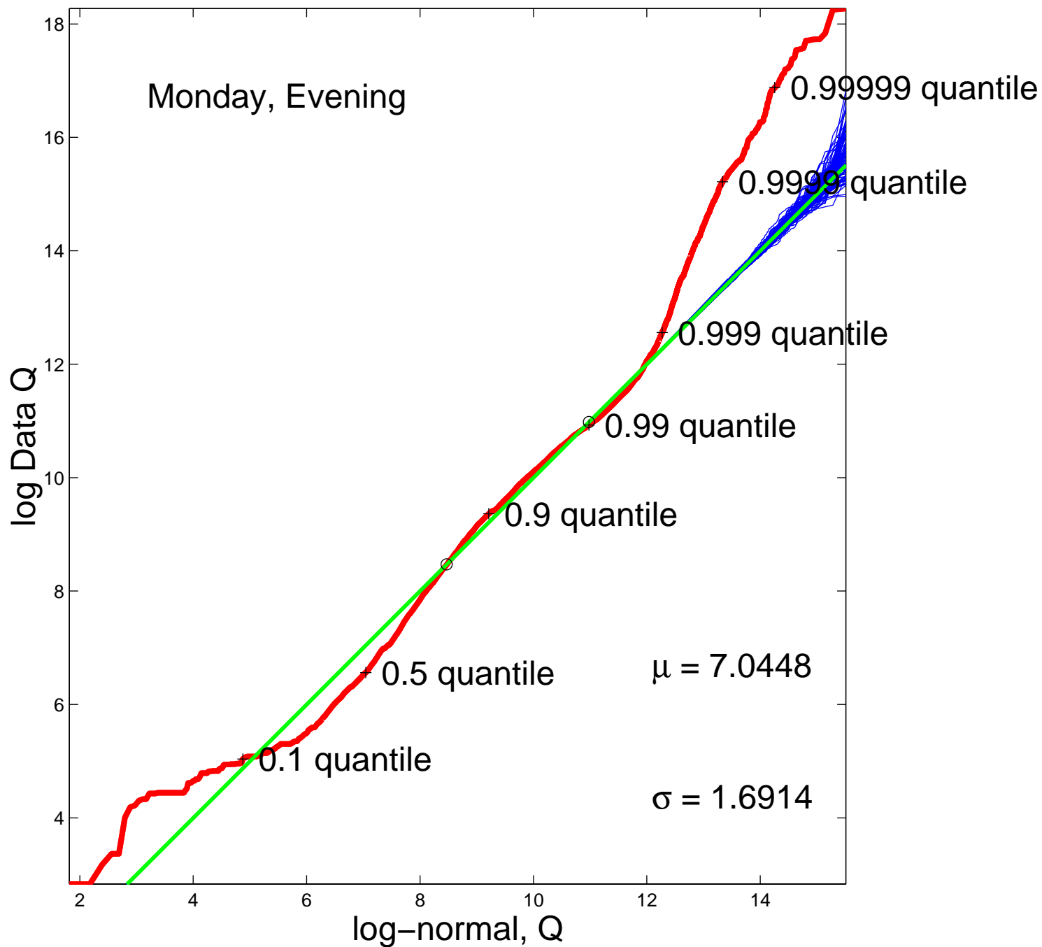
HTTP R. S., log-normal Q-Q, 0.8 & 0.99 quant. matched, n = 3575530
