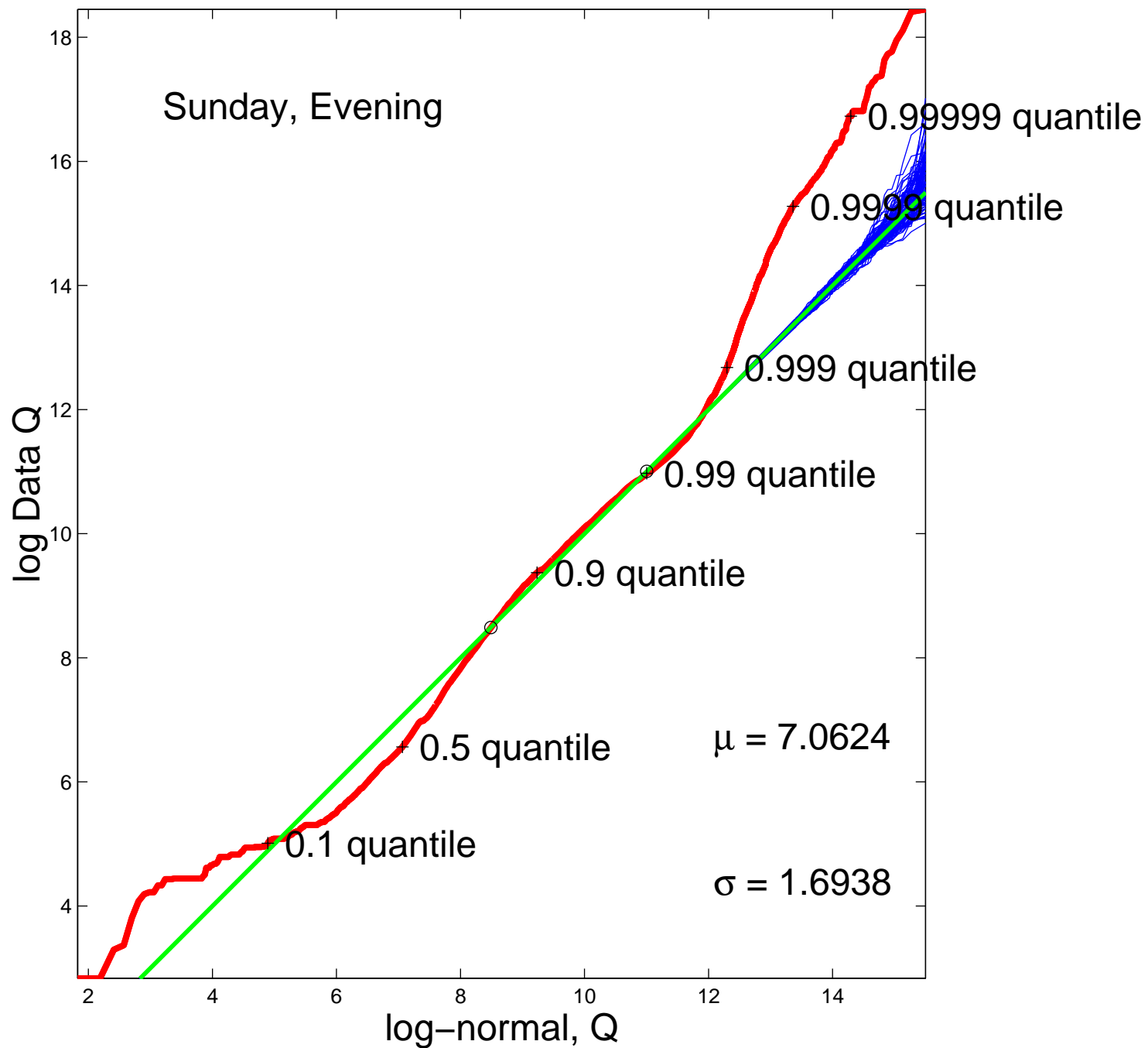
HTTP R. S., log-normal Q-Q, 0.8 & 0.99 quant. matched, n = 3147247
