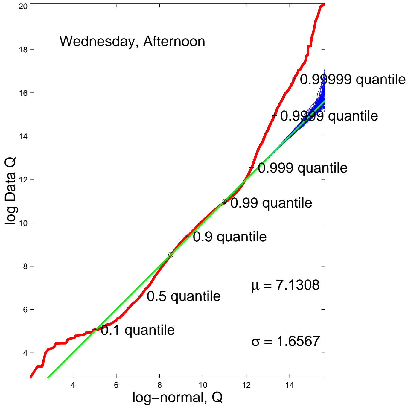
HTTP R. S., log-normal Q-Q, 0.8 & 0.99 quant. matched, n = 7136393
