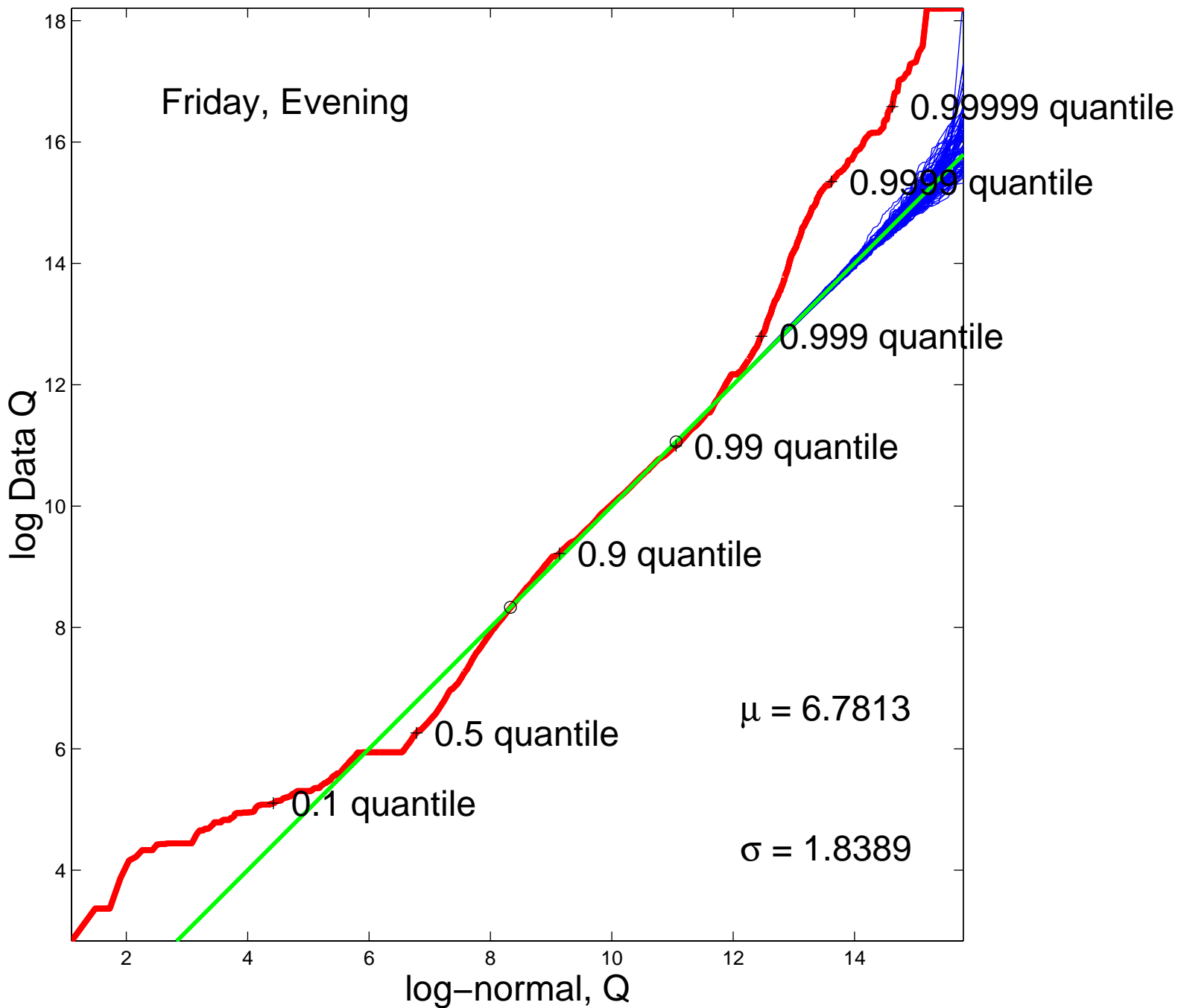
HTTP R. S., log-normal Q-Q, 0.8 & 0.99 quant. matched, n = 2087324
