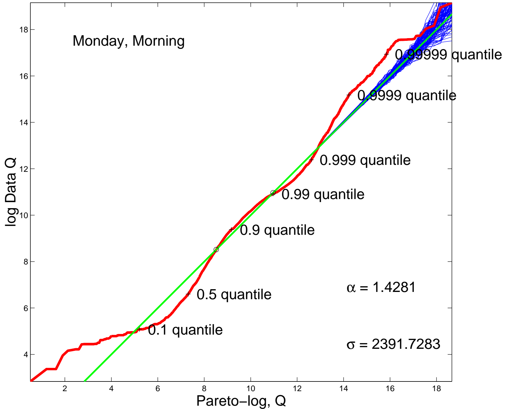
HTTP R. S., Pareto Q-Q, 0.8 & 0.99 quant. matched, n = 5621502
