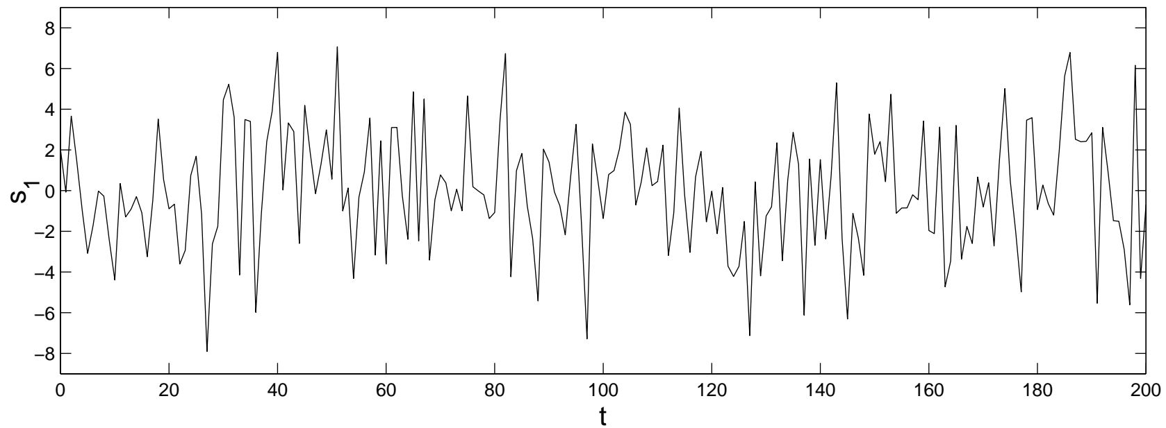
Gaussian Noise & Bimodal, PCA decomposition, PC1
