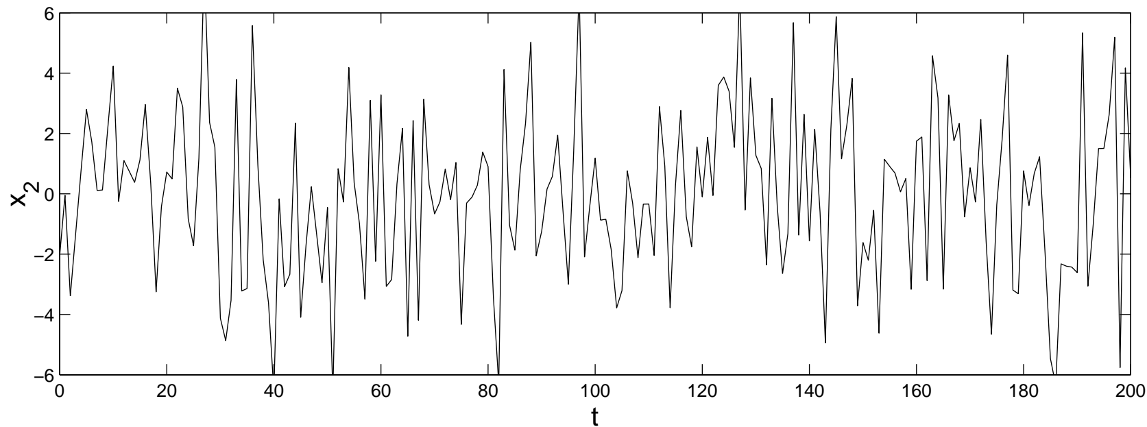
Gaussian Noise & Bimodal, Mixed signal x_2
