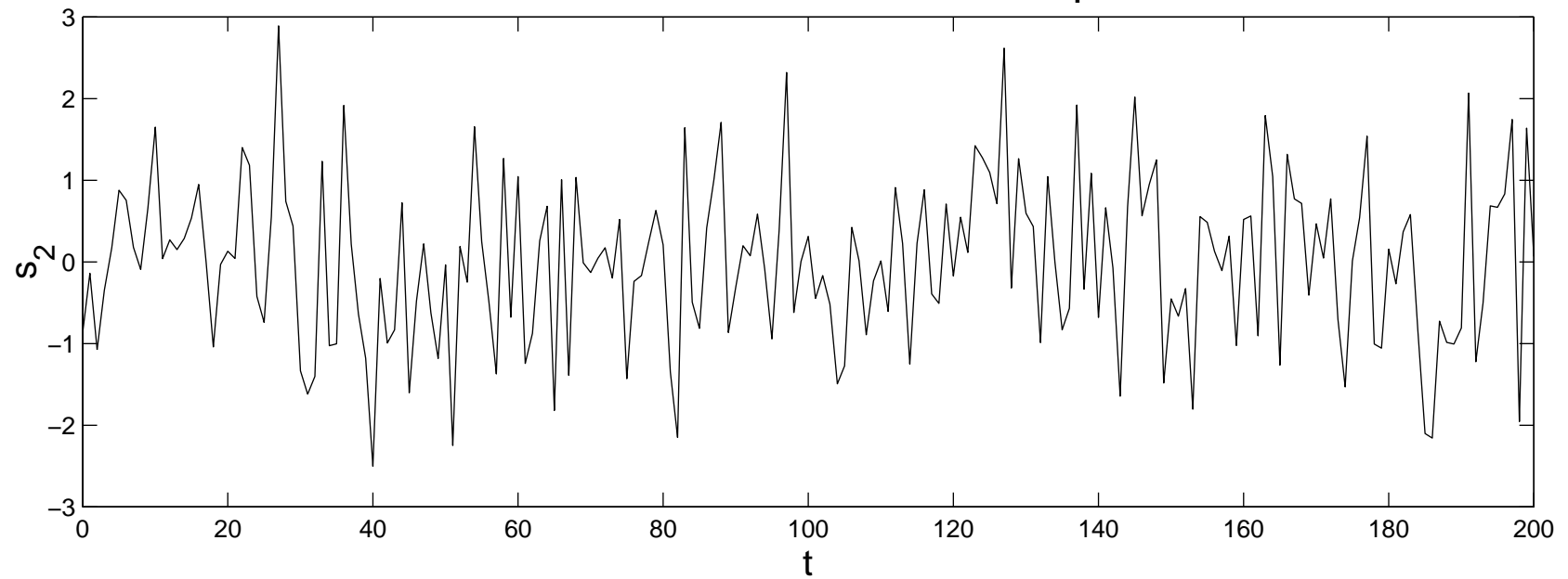
Gaussian Noise & Bimodal, ICA decomposition, IC2
