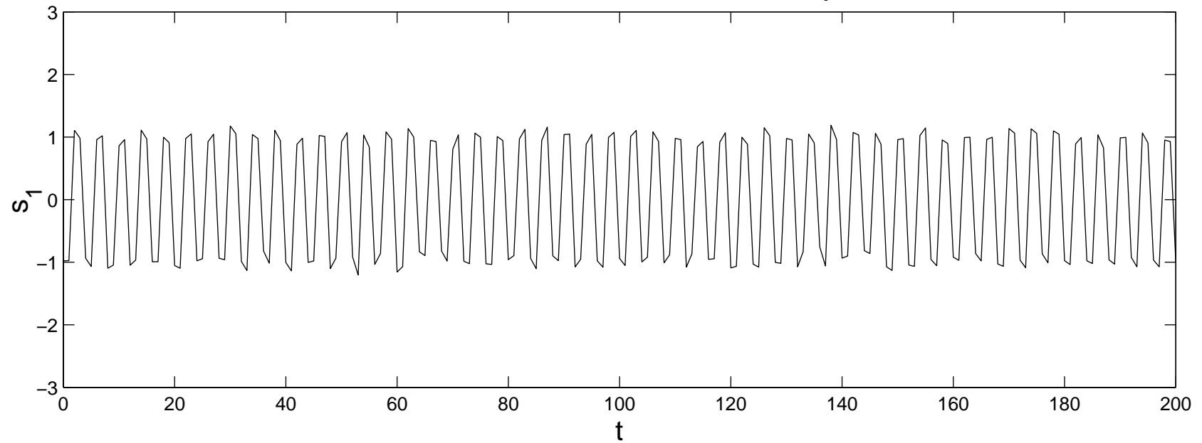
Gaussian Noise & Bimodal, ICA decomposition, IC1
