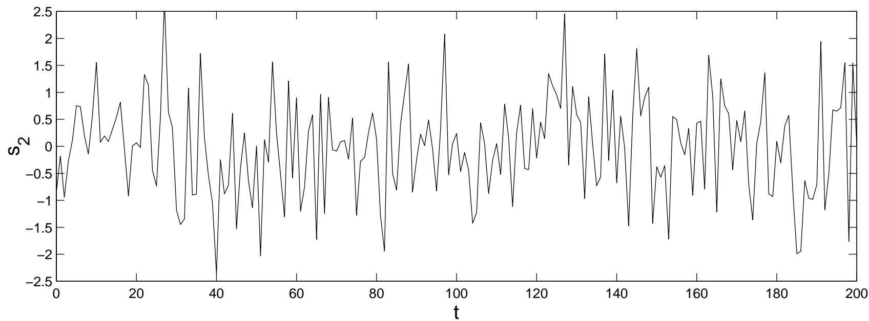
Gaussian Noise & Bimodal, Original signal s_2
