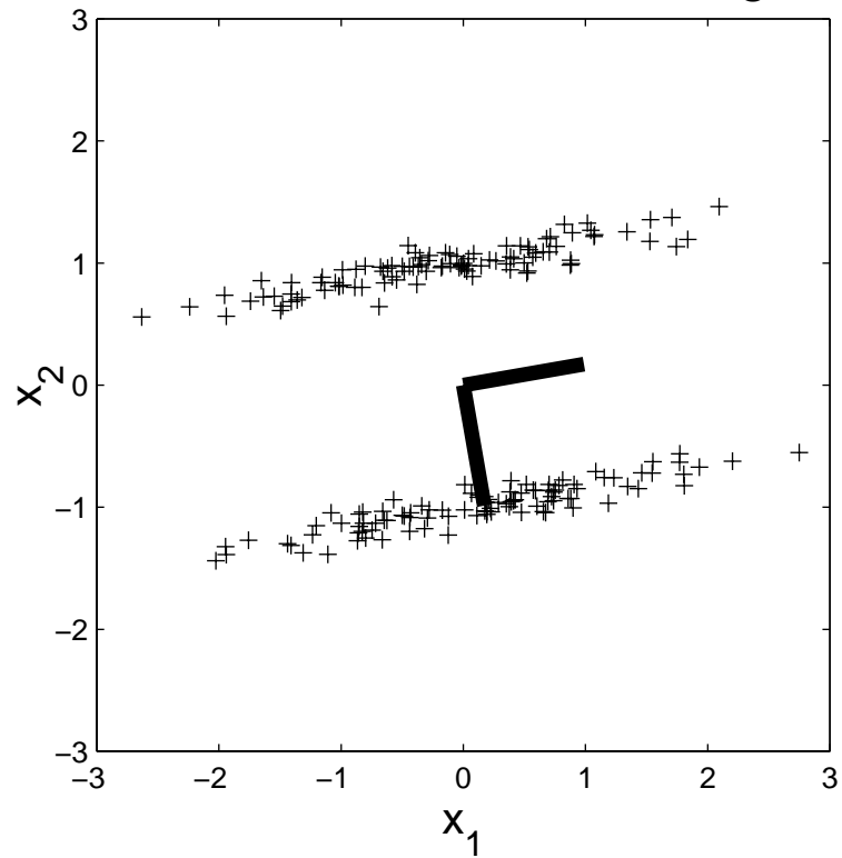
Gaussian Noise & Bimodal, ICA eigenvectors
