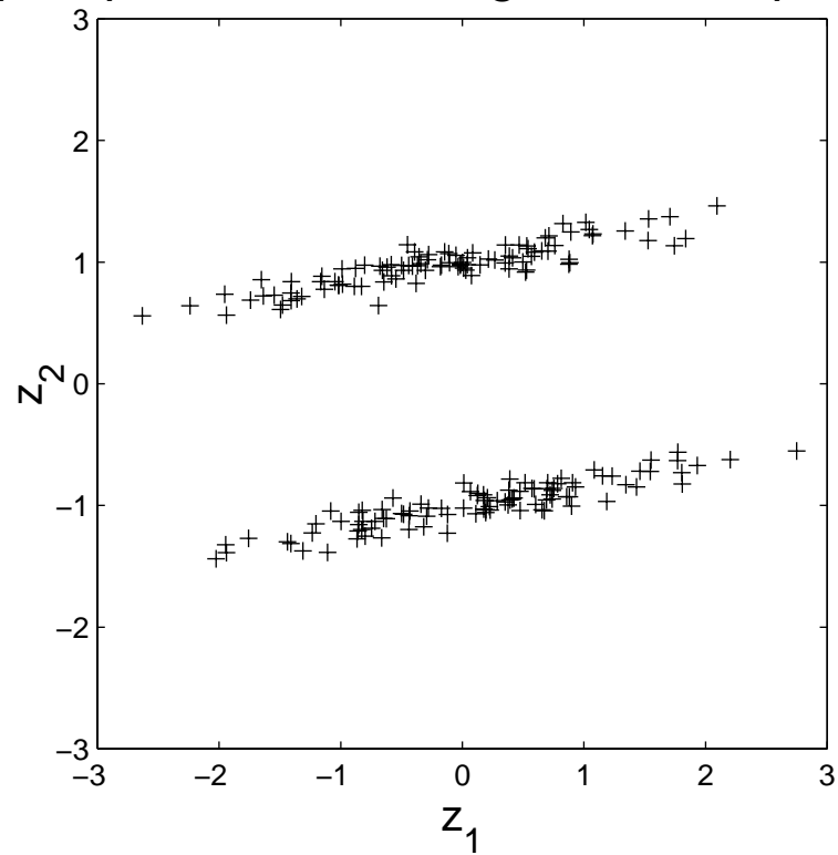
Gaussian Noise & Bimodal, Mixed Signal Scatterplot Sphered Mixed Signal Scatterplot
