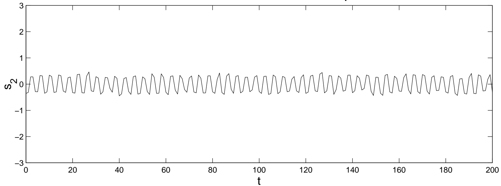
Gaussian Noise & Bimodal, PCA decomposition, PC2
