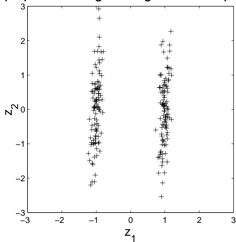
Gaussian Noise & Bimodal, Original Signal Scatterplot Sphered Original Signal Scatterplot
