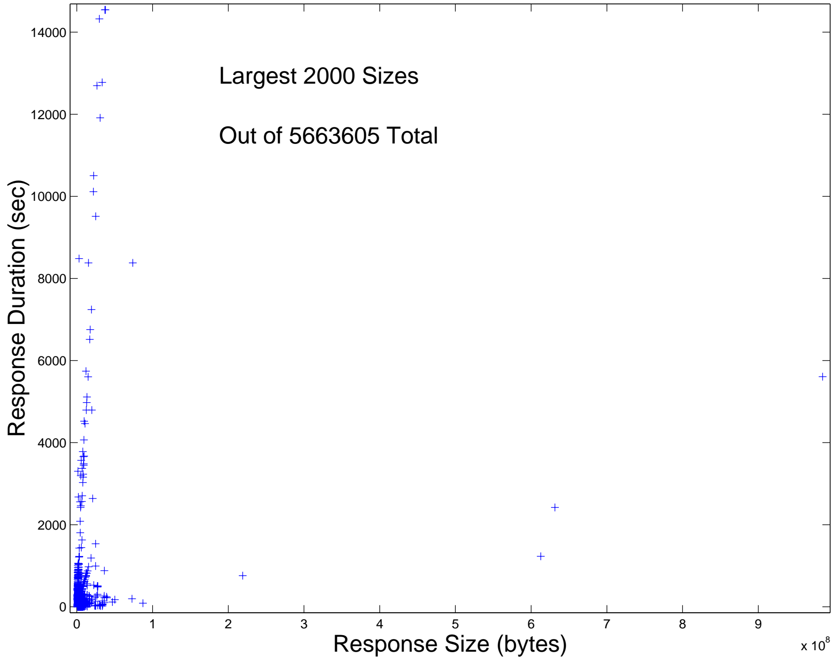
HTTP Response Size Scatterplot, Thursday, Morning
