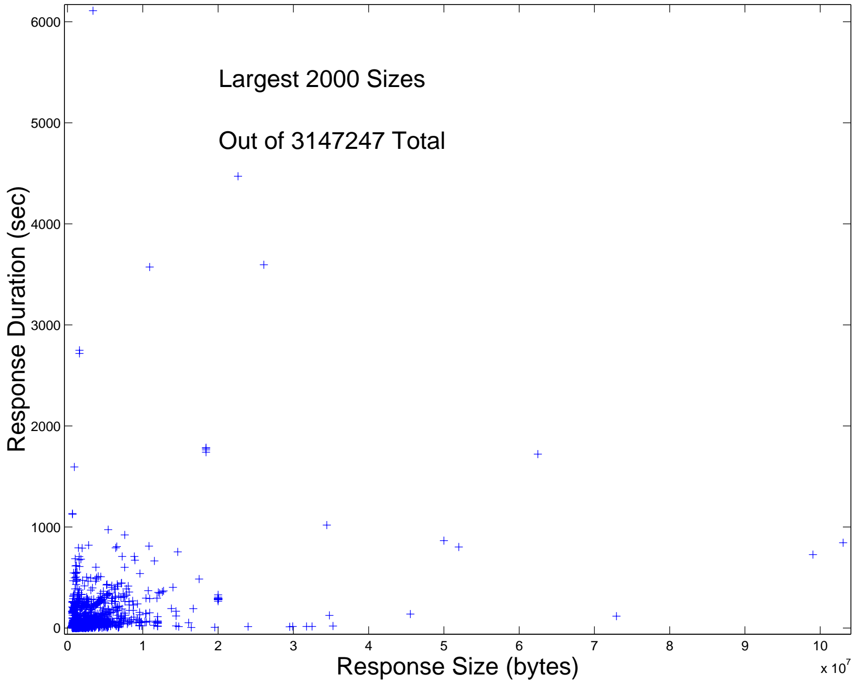
HTTP Response Size Scatterplot, Sunday, Evening
