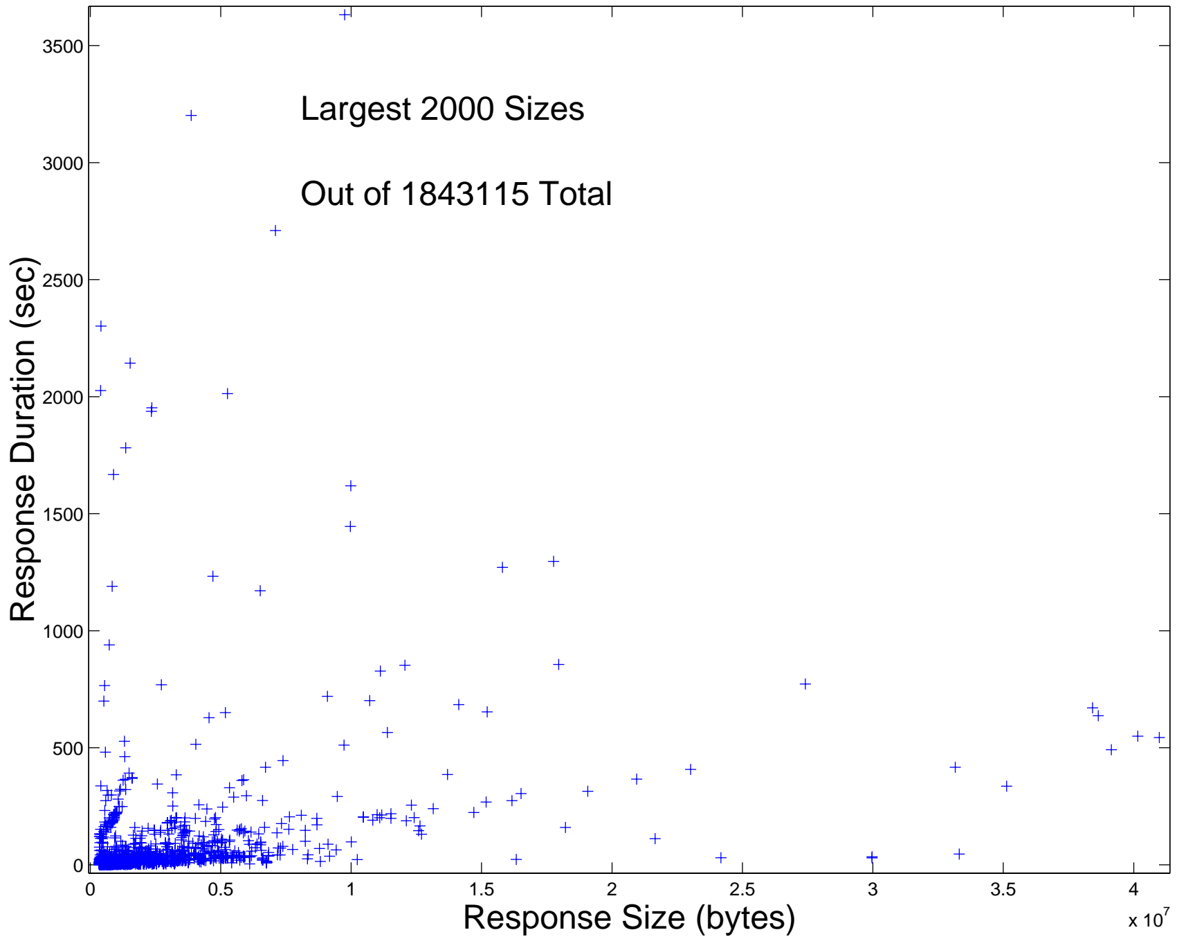
HTTP Response Size Scatterplot, Saturday, Evening
