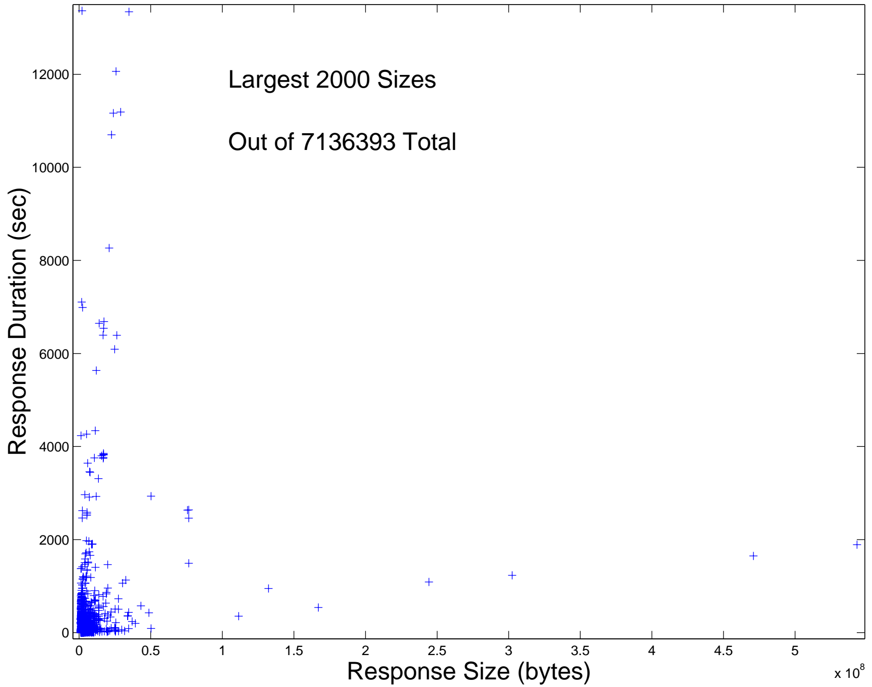
HTTP Response Size Scatterplot, Wednesday, Afternoon
