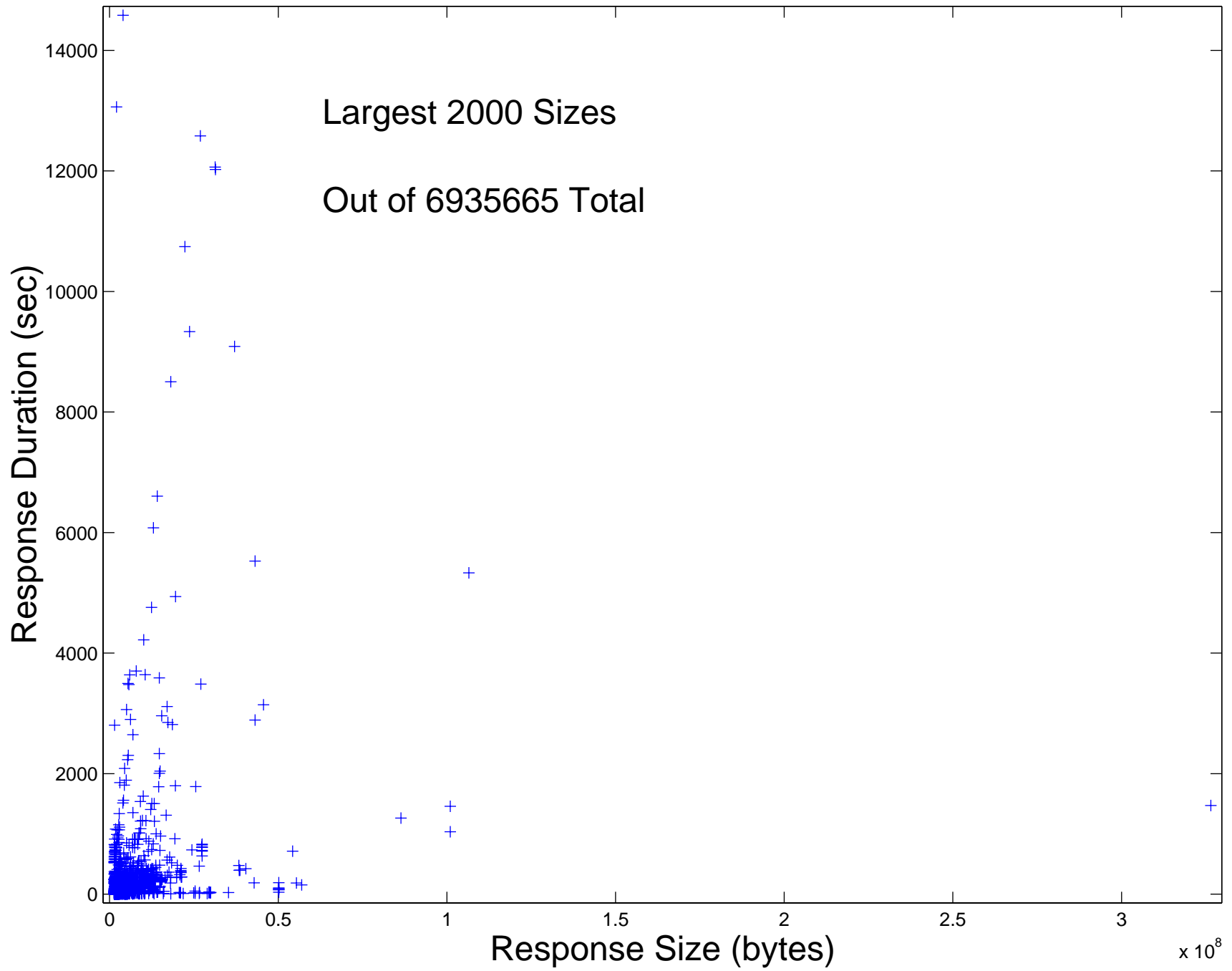
HTTP Response Size Scatterplot, Monday, Afternoon
