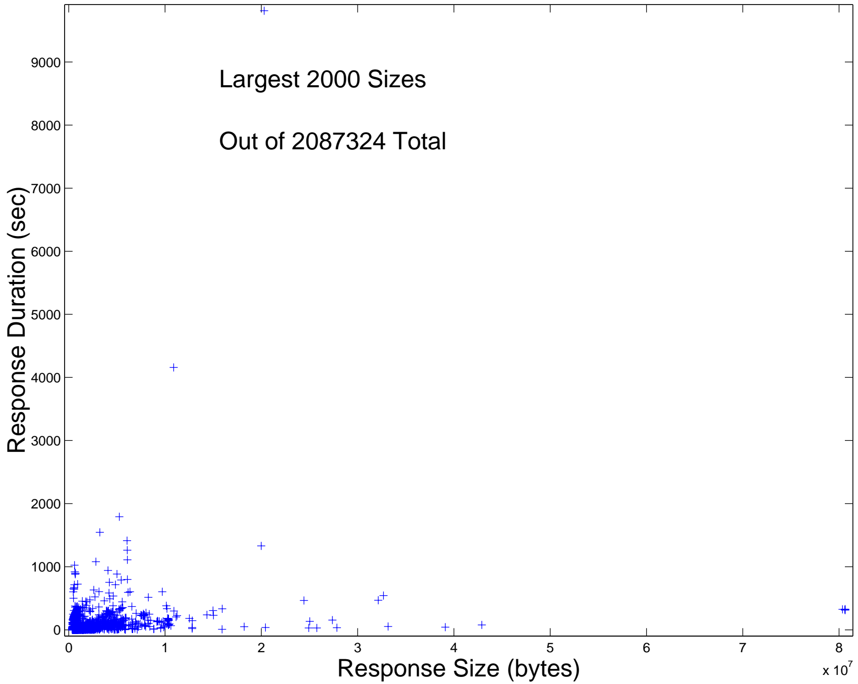
HTTP Response Size Scatterplot, Friday, Evening
