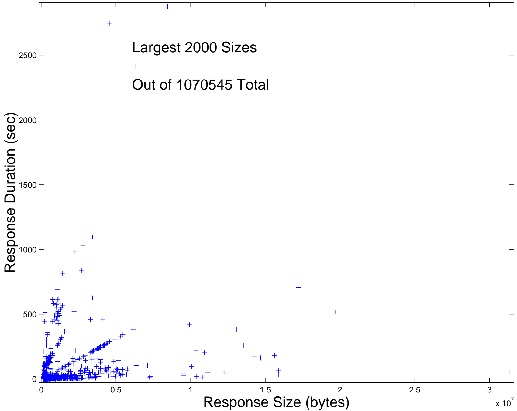
HTTP Response Size Scatterplot, Sunday, Morning
