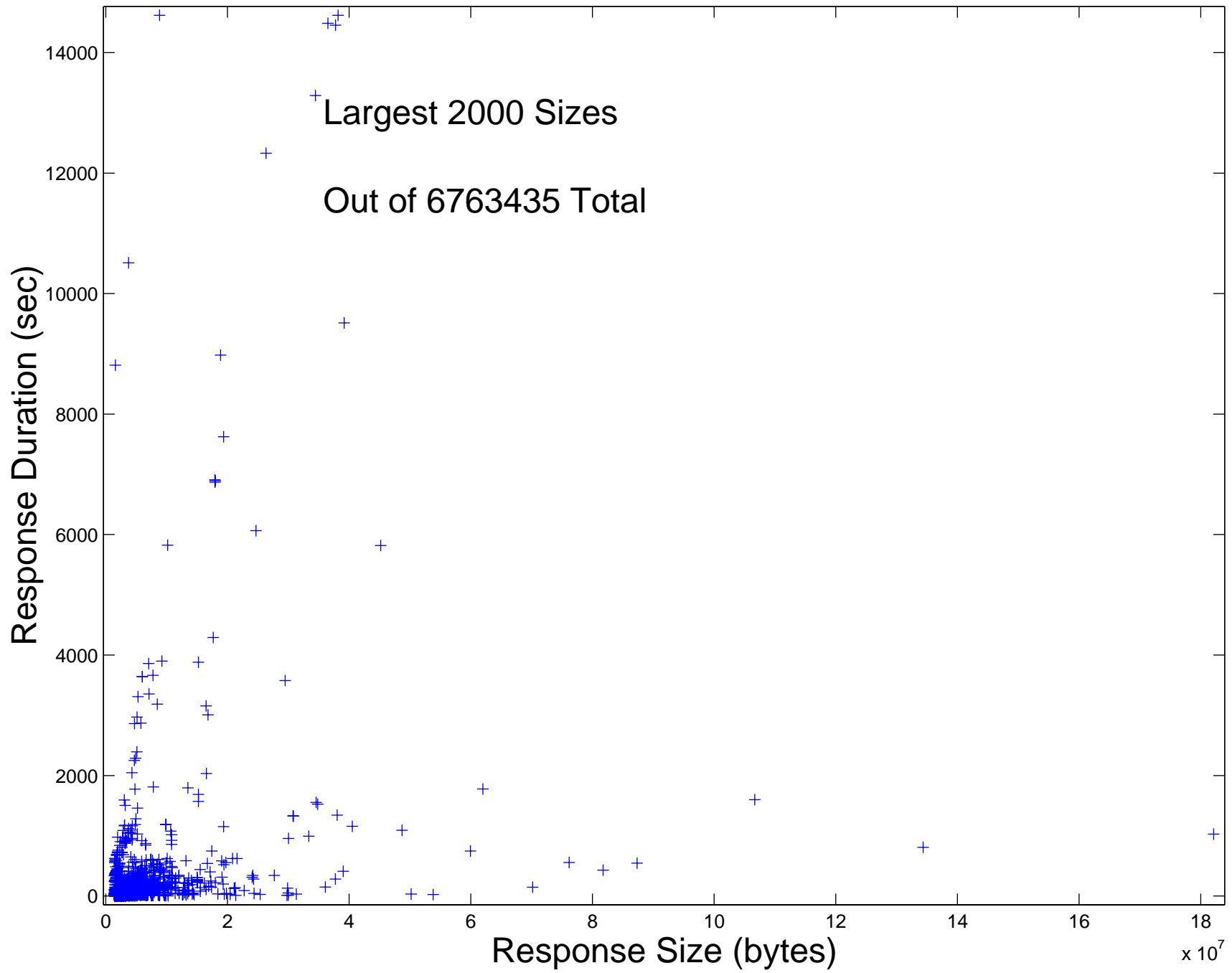
HTTP Response Size Scatterplot, Tuesday, Afternoon
