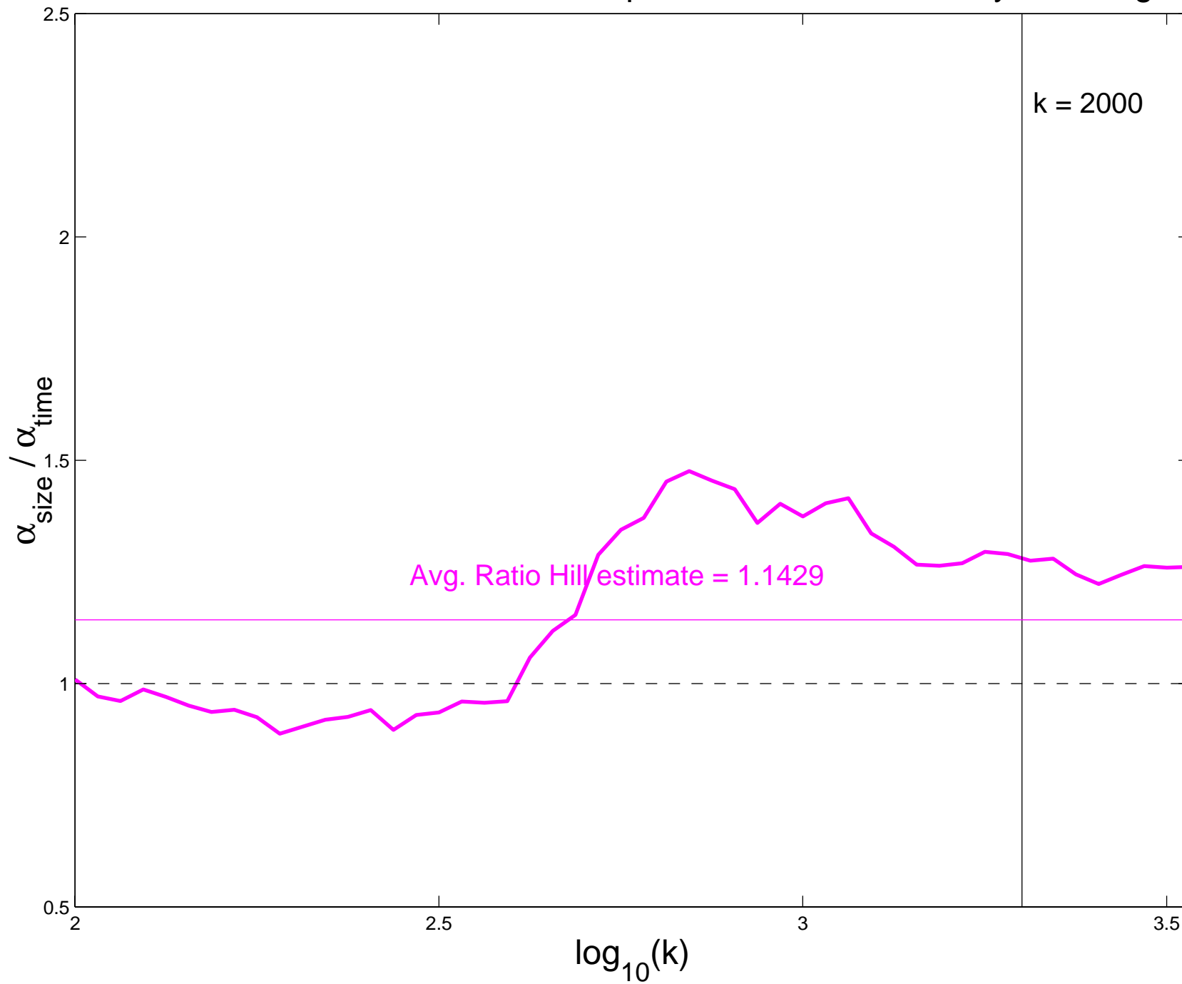
Ratio Hill estimates for HTTP Response Durations, Sunday, Evening
