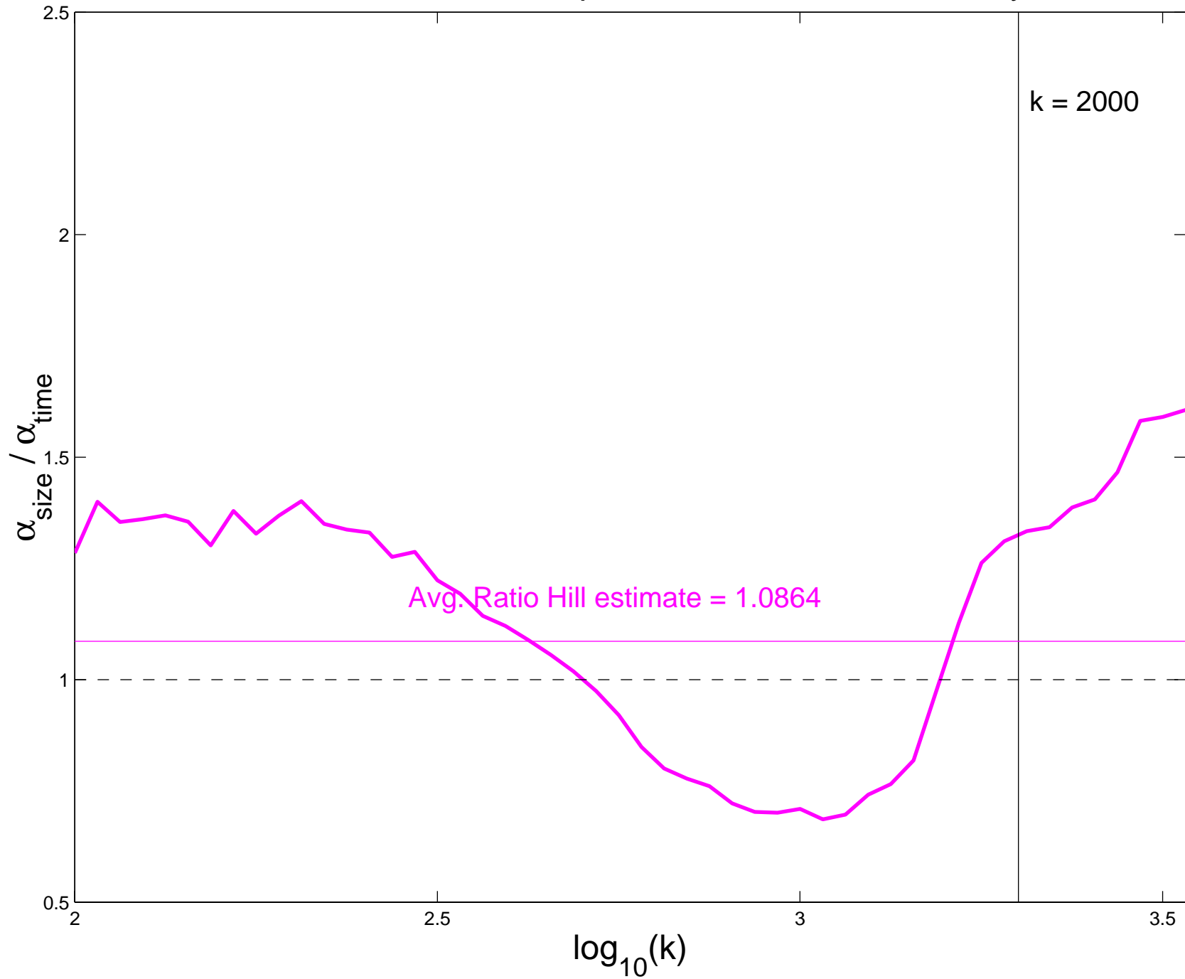
Ratio Hill estimates for HTTP Response Durations, Wednesday, Afternoon
