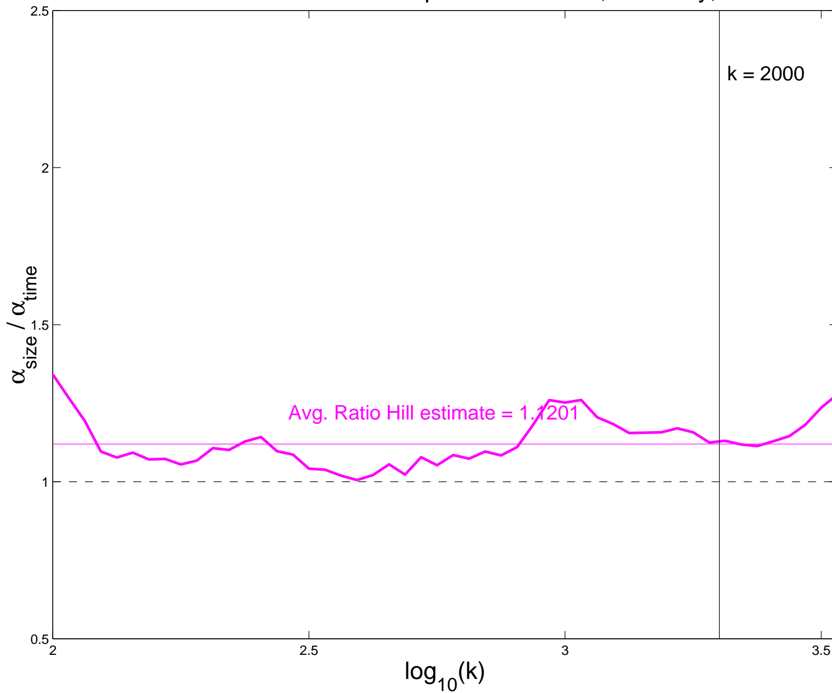
Ratio Hill estimates for HTTP Response Durations, Saturday, Afternoon
