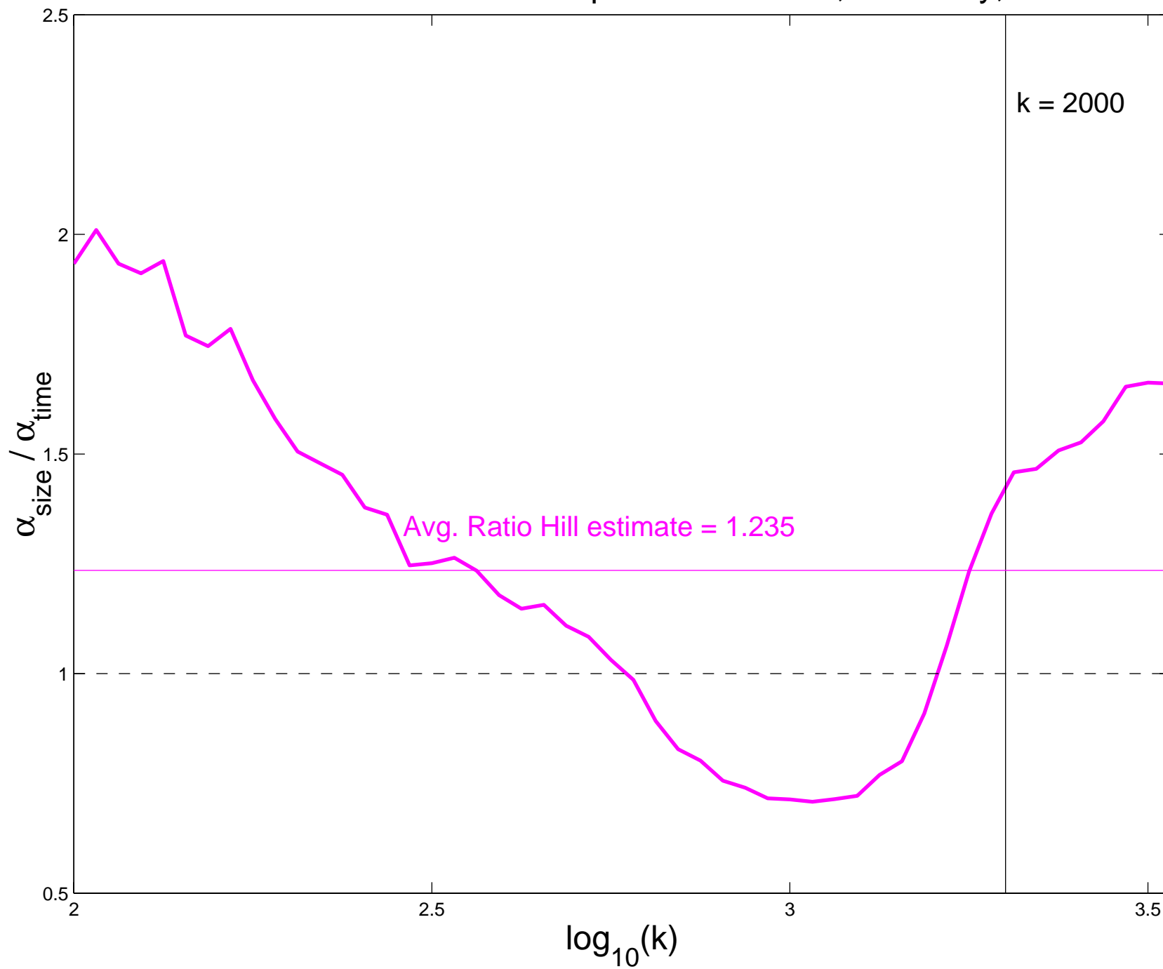
Ratio Hill estimates for HTTP Response Durations, Thursday, Afternoon
