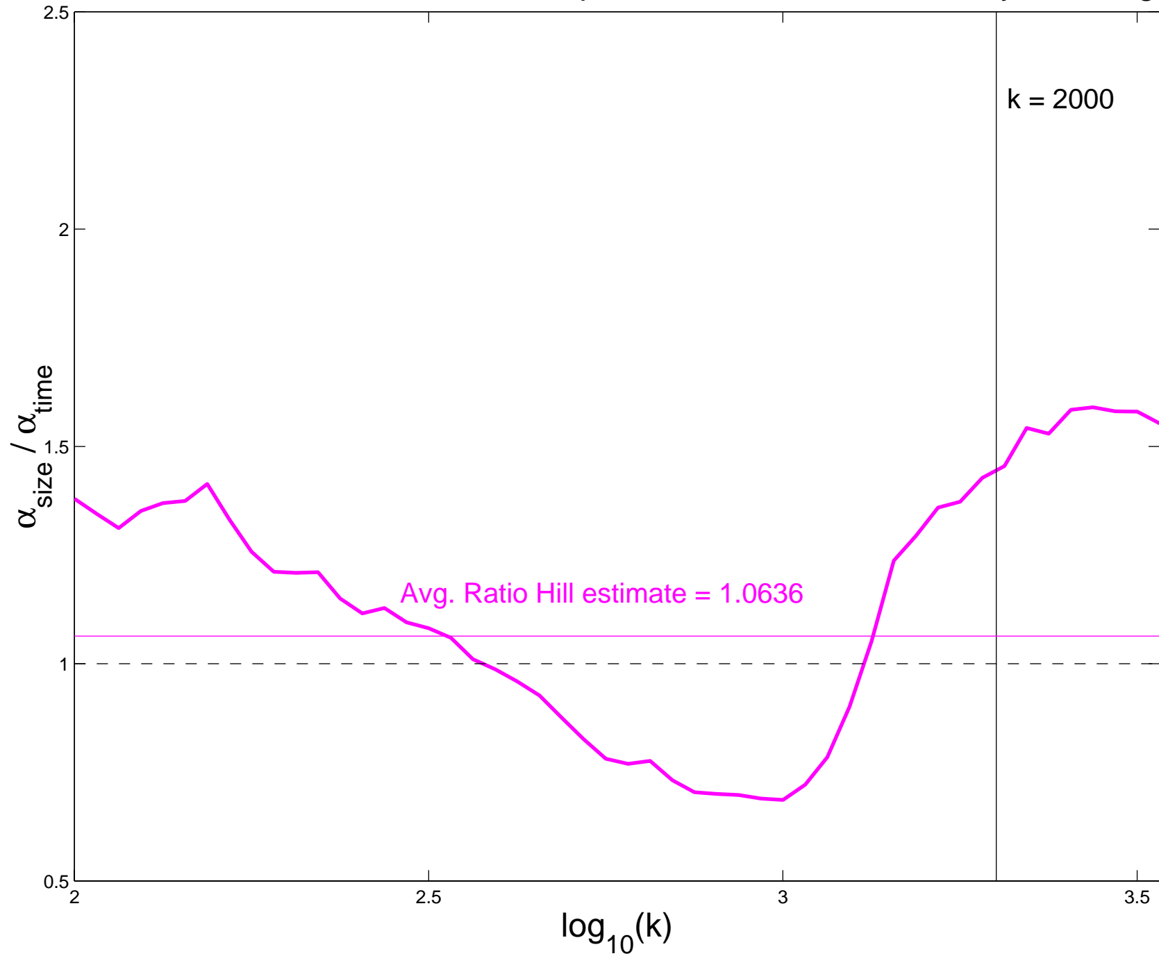
Ratio Hill estimates for HTTP Response Durations, Wednesday, Morning
