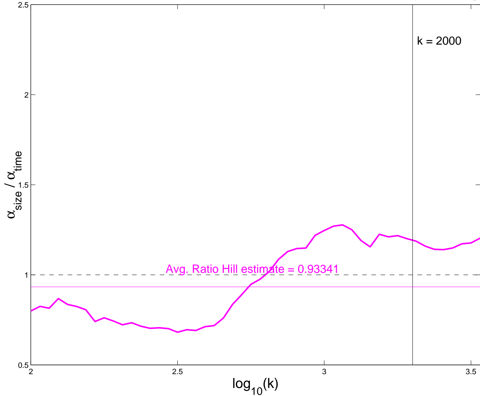
Ratio Hill estimates for HTTP Response Durations, Wednesday, Evening
