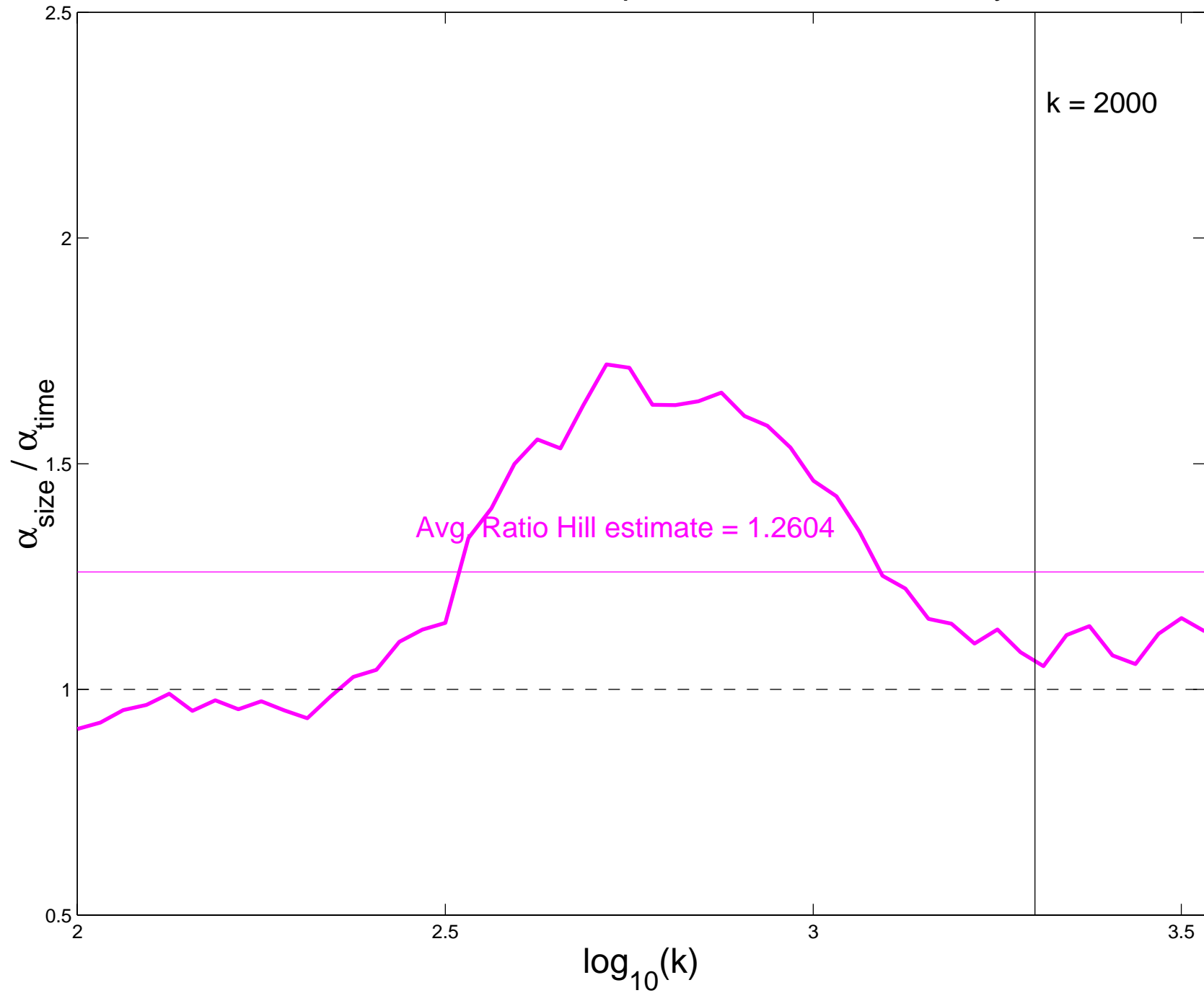
Ratio Hill estimates for HTTP Response Durations, Sunday, Afternoon
