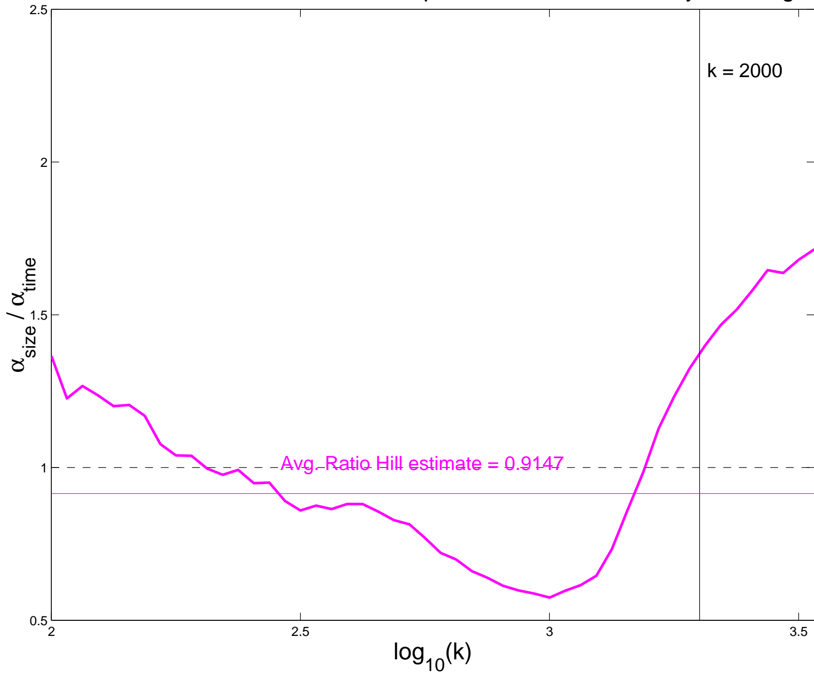
Ratio Hill estimates for HTTP Response Durations, Tuesday, Morning
