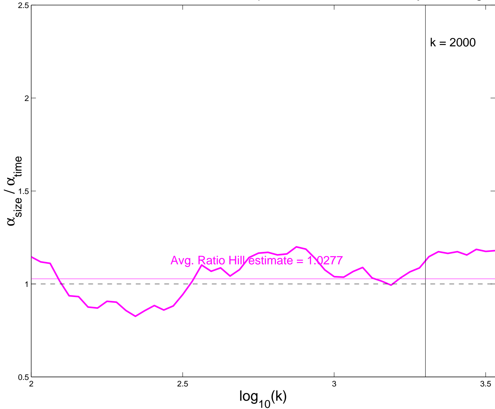
Ratio Hill estimates for HTTP Response Durations, Tuesday, Evening
