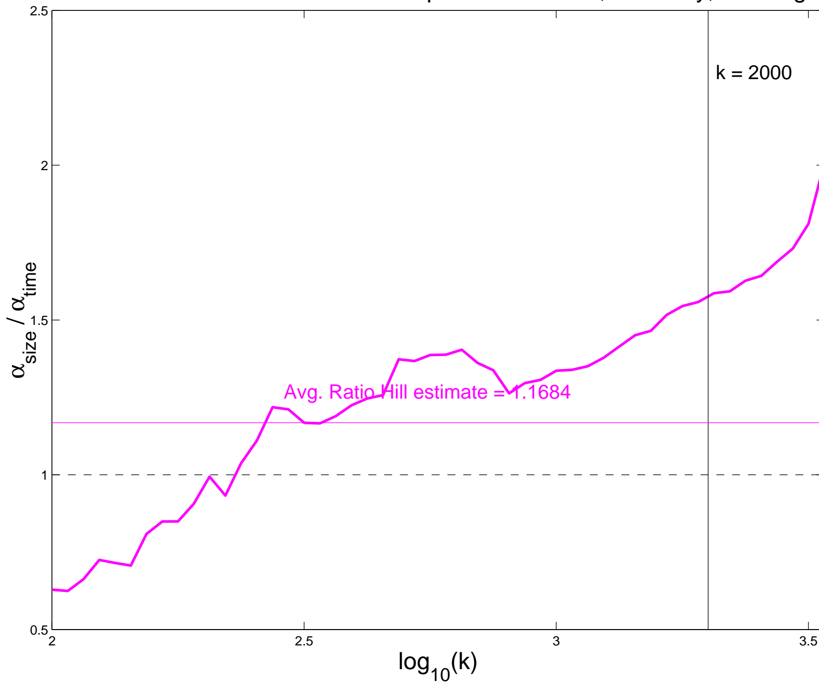
Ratio Hill estimates for HTTP Response Durations, Saturday, Morning
