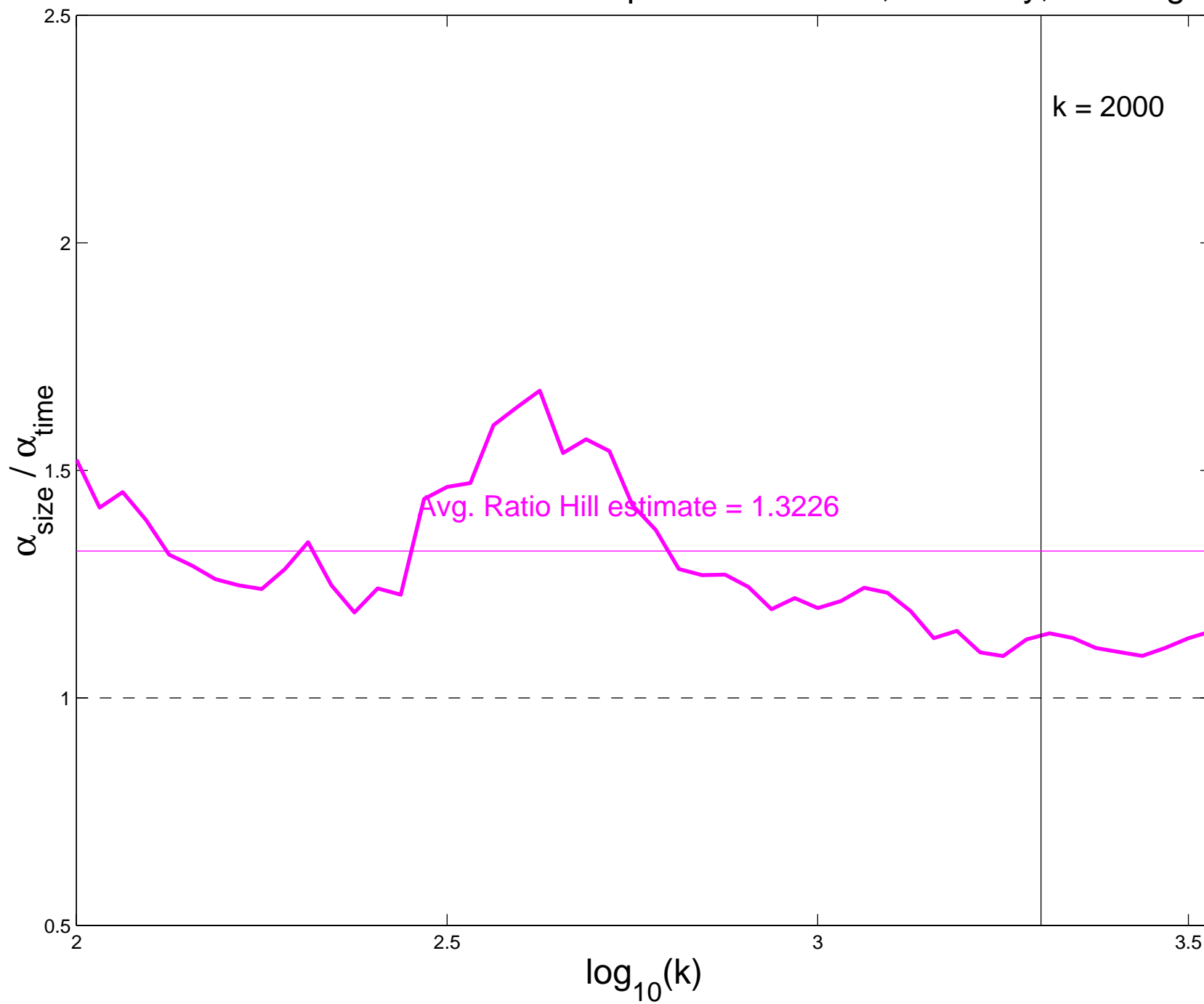
Ratio Hill estimates for HTTP Response Durations, Saturday, Evening
