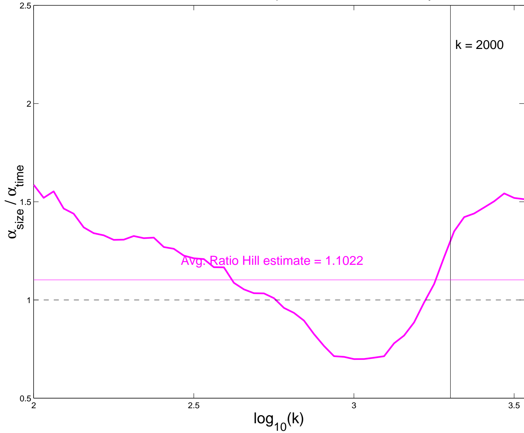
Ratio Hill estimates for HTTP Response Durations, Friday, Afternoon
