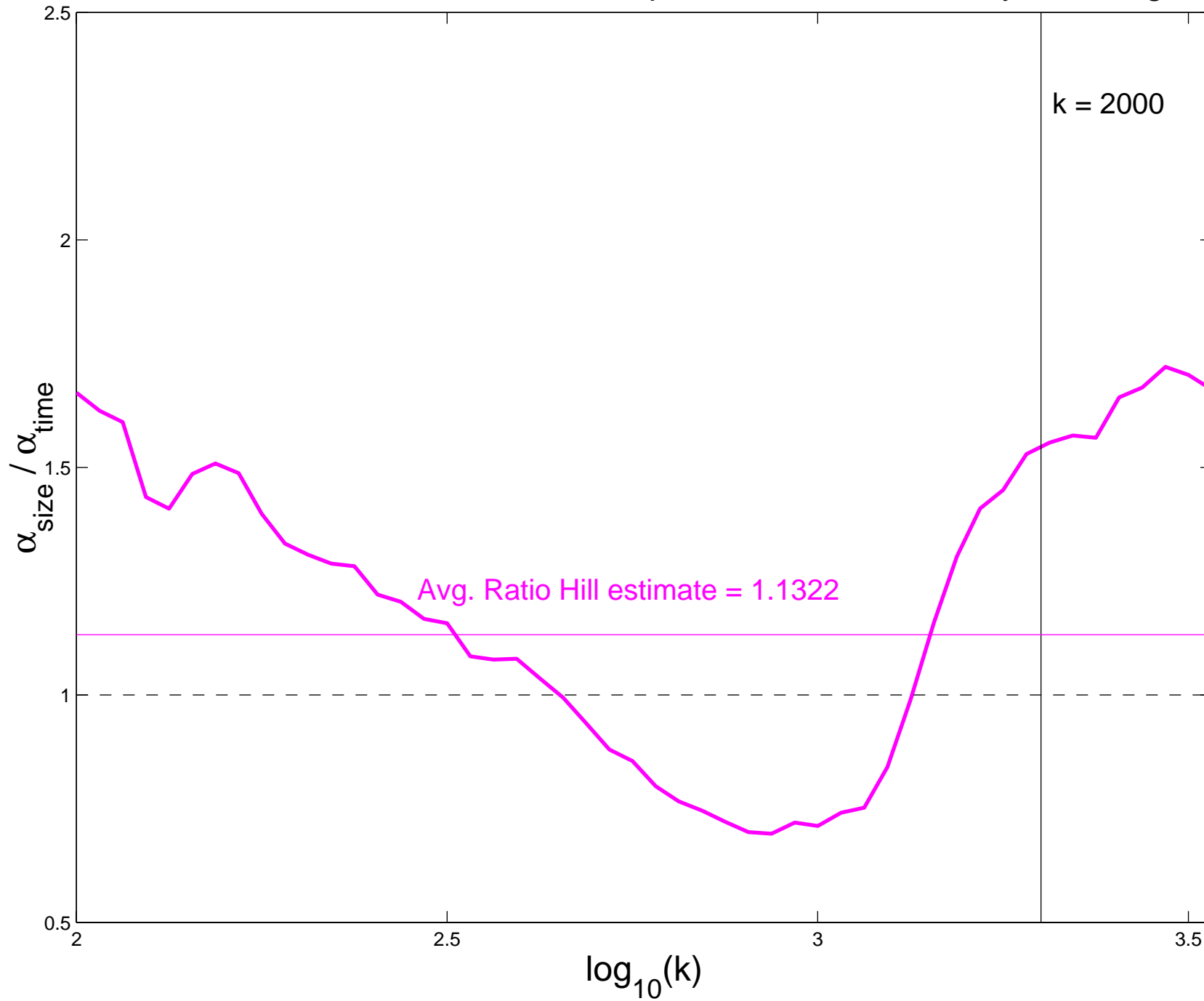
Ratio Hill estimates for HTTP Response Durations, Friday, Morning
