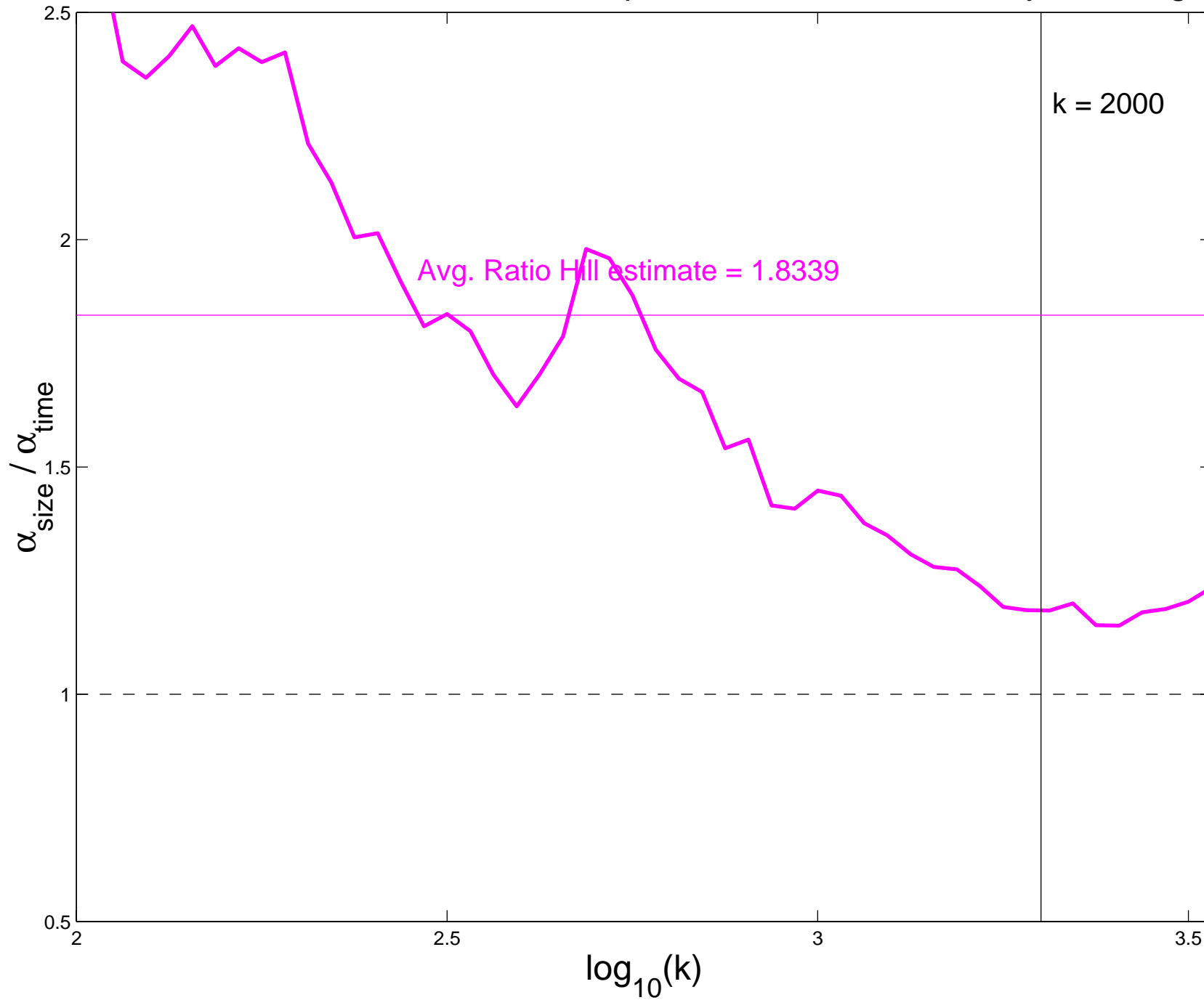
Ratio Hill estimates for HTTP Response Durations, Thursday, Evening
