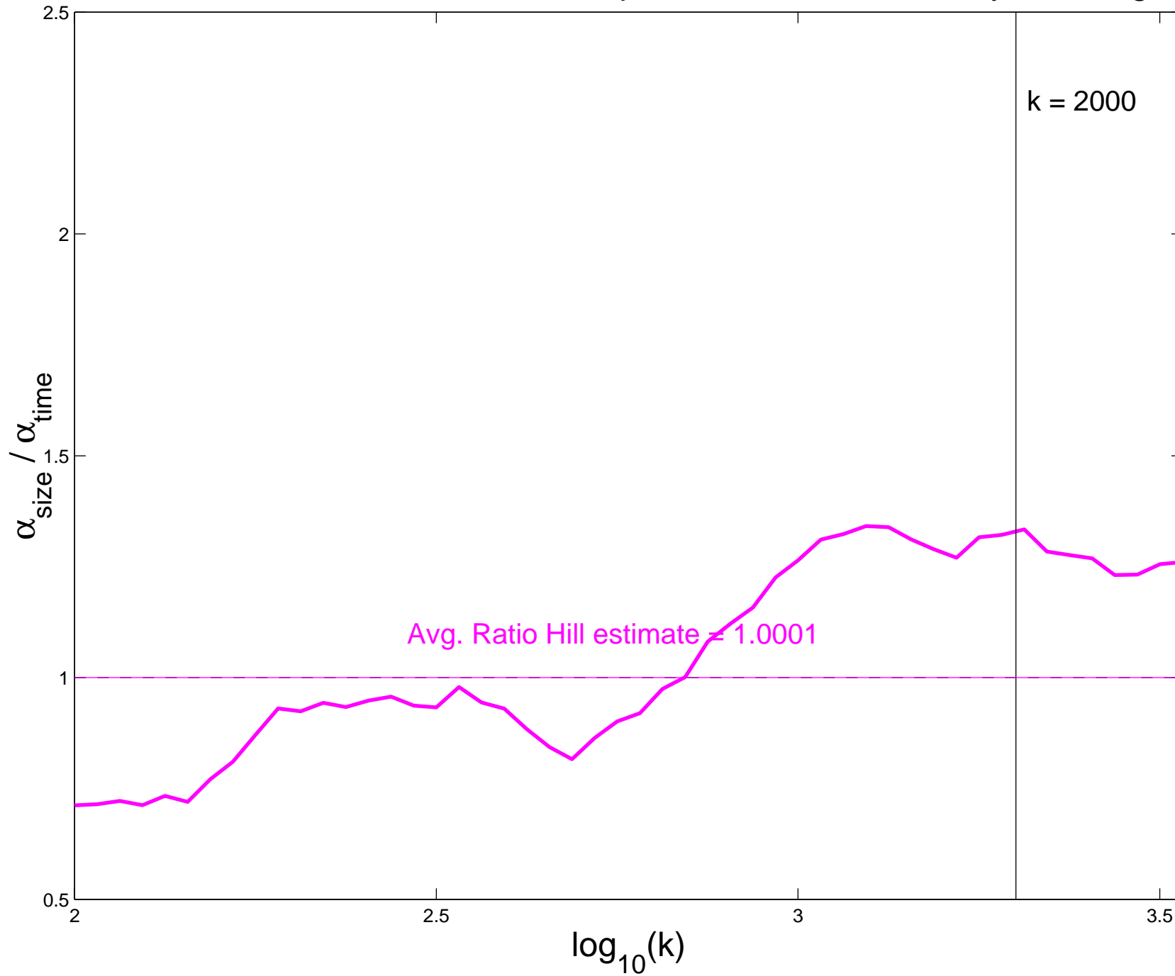
Ratio Hill estimates for HTTP Response Durations, Monday, Evening
