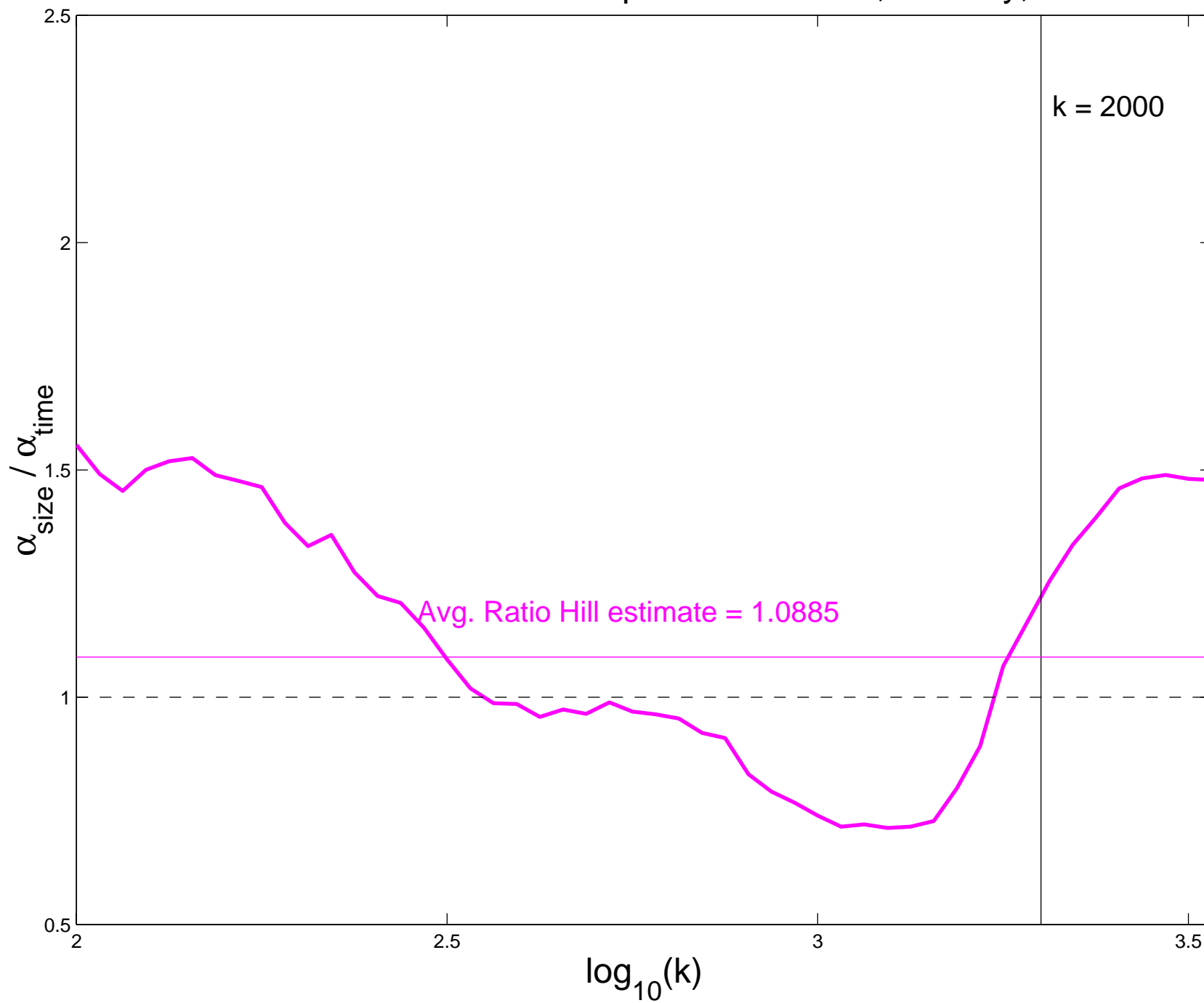
Ratio Hill estimates for HTTP Response Durations, Monday, Afternoon
