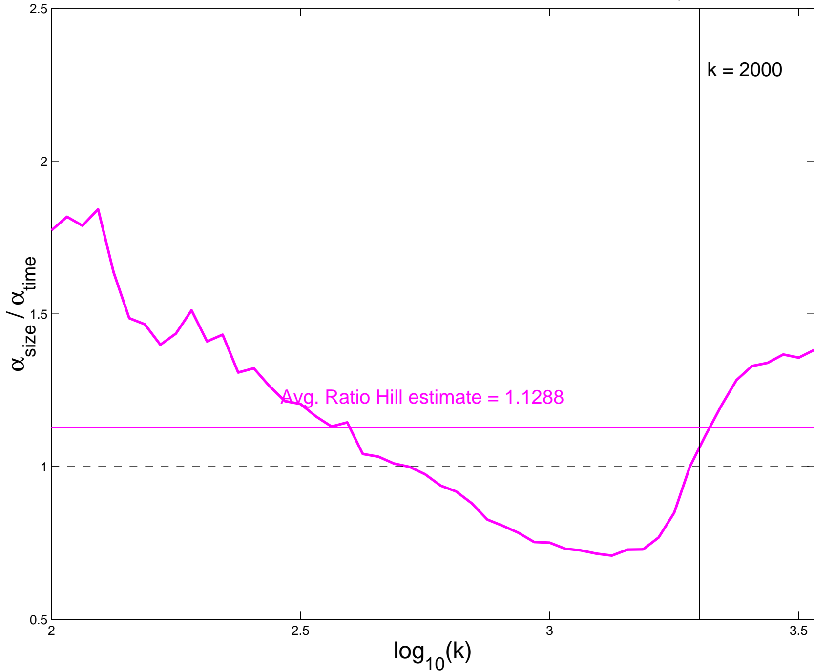
Ratio Hill estimates for HTTP Response Durations, Tuesday, Afternoon
