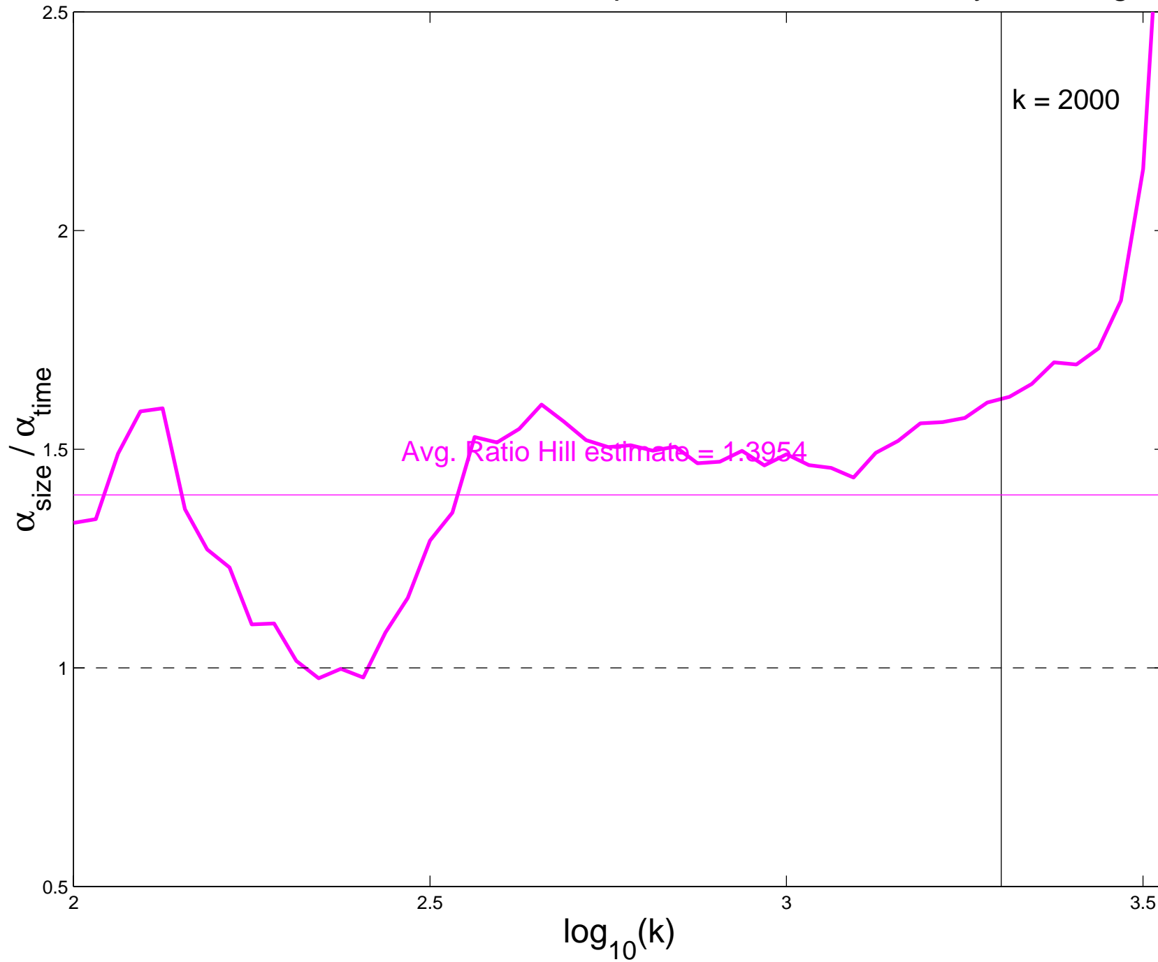
Ratio Hill estimates for HTTP Response Durations, Sunday, Morning
