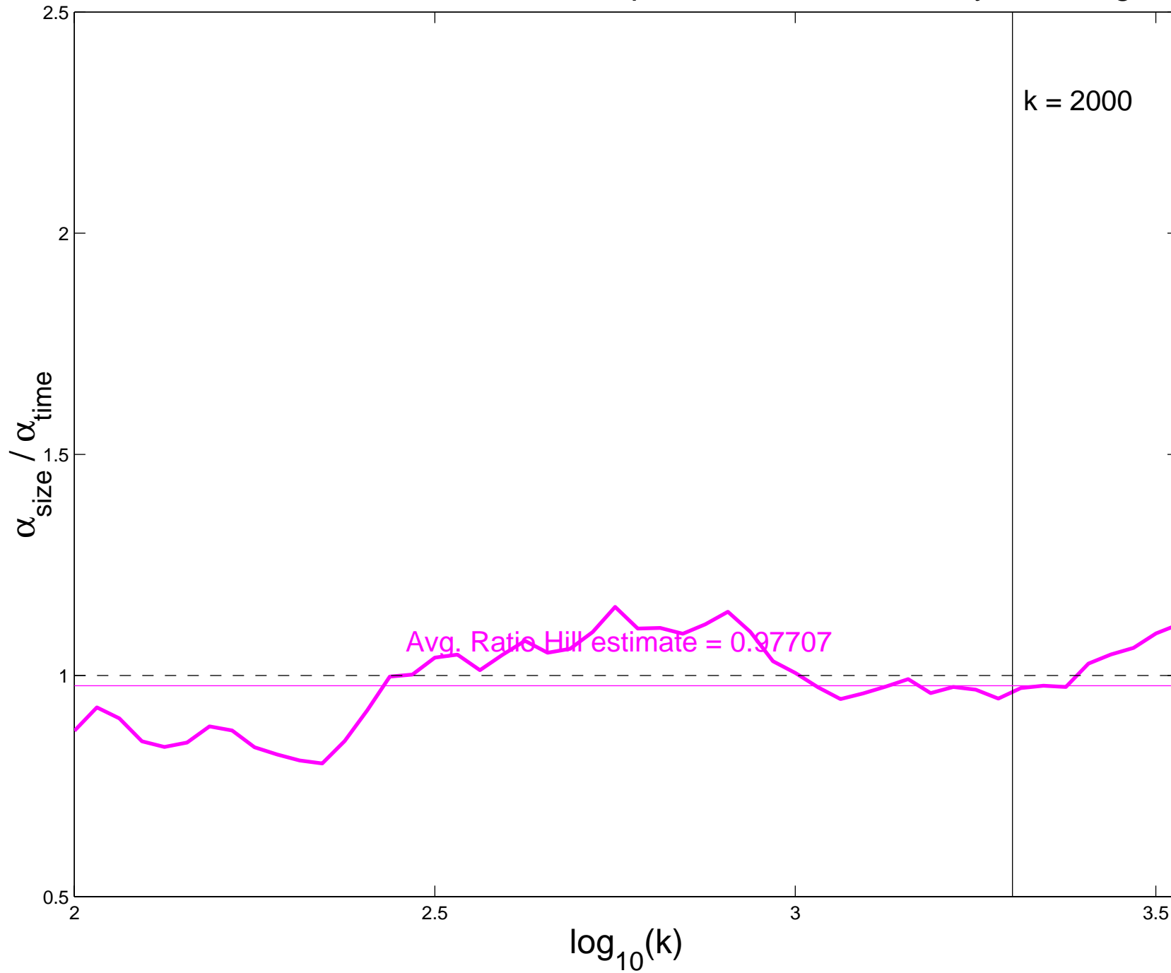
Ratio Hill estimates for HTTP Response Durations, Friday, Evening
