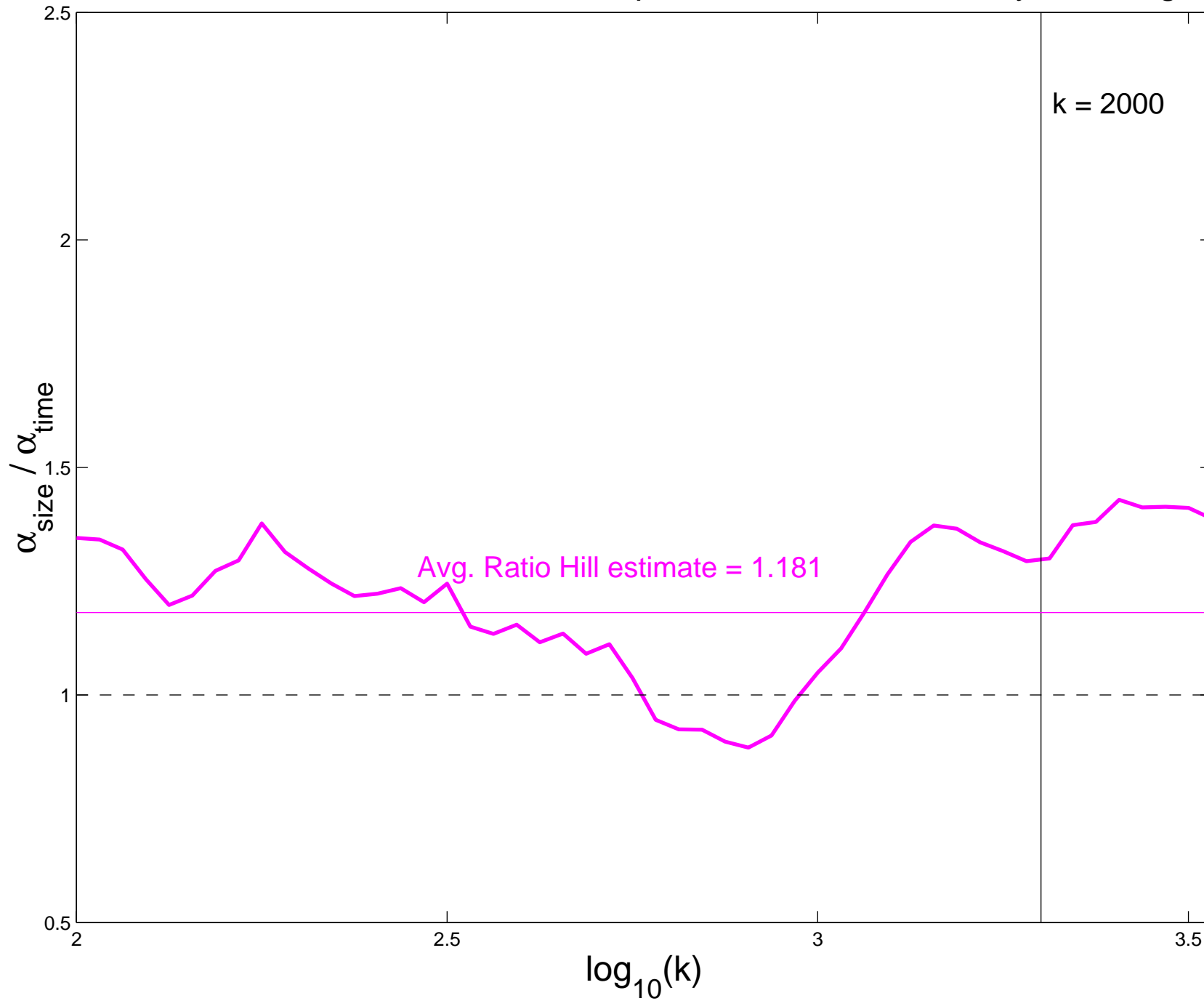
Ratio Hill estimates for HTTP Response Durations, Monday, Morning
