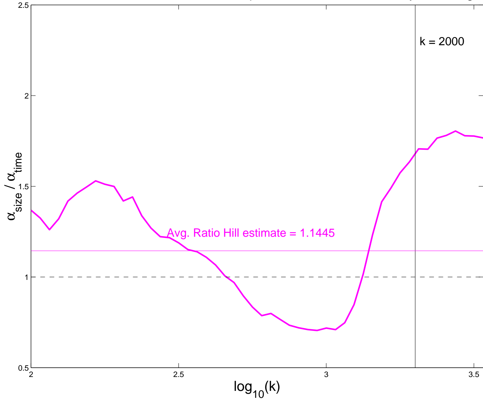
Ratio Hill estimates for HTTP Response Durations, Thursday, Morning
