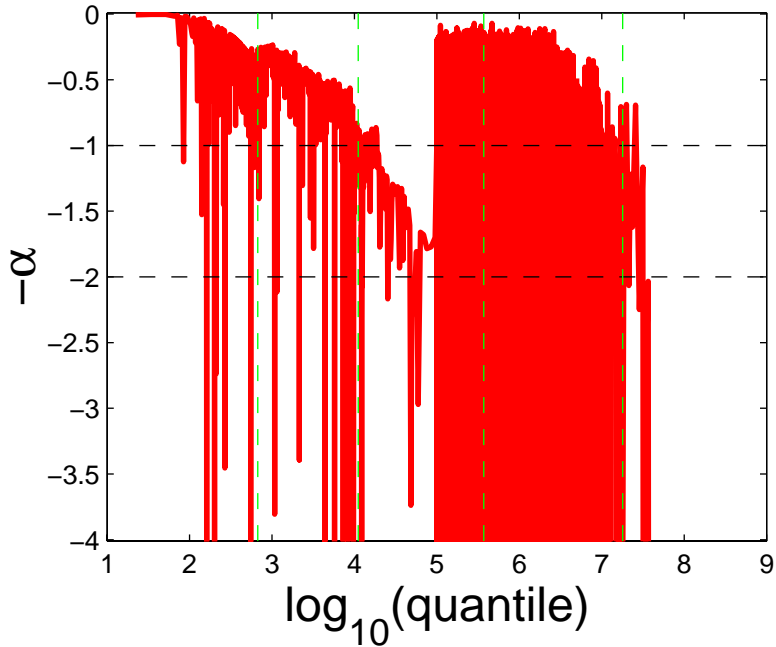
Corresponding Slopes of log-log CCDF
