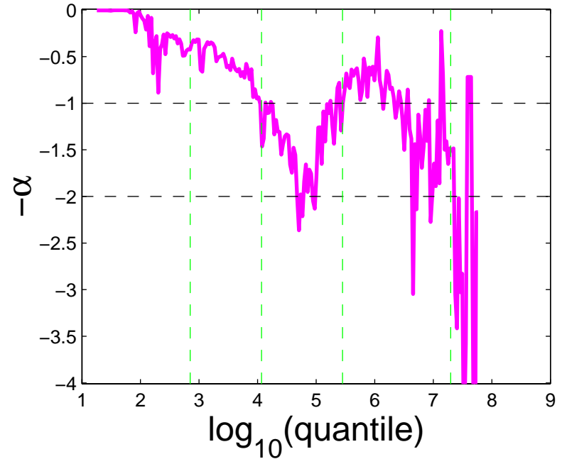
\Delta = 0.03 Slopes of log-log CCDF
