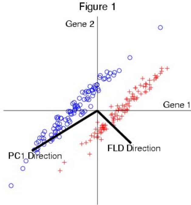
Figure 1: Hypothetical 2 gene example showing how PCA directions can be wrong for source adjustment, thereby motivating methods based on discrimination ideas. Circles represent samples from source one and '+' represents samples from source 2.
