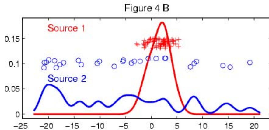
Figure 4: Application of DWD to same data as in Figures 3, 5 and 6. Shows both good separation, and also reasonable subpopulation shape for mean shift adjustment
