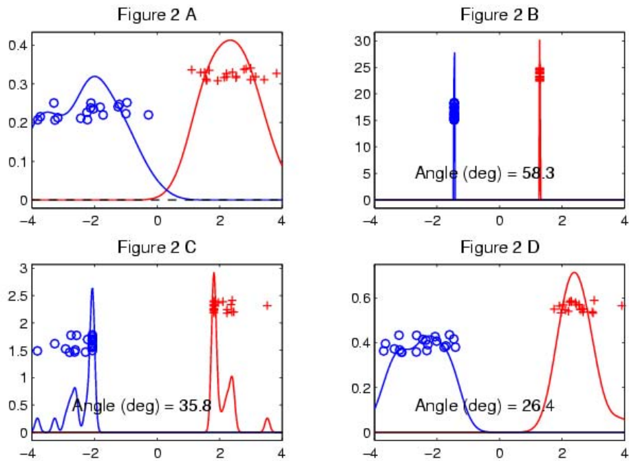
Figure 2: 50 dimensional/gene Gaussian hypothetical example, to illustrate HDLSS failing of FLD, and superior performance of DWD over SVM.
