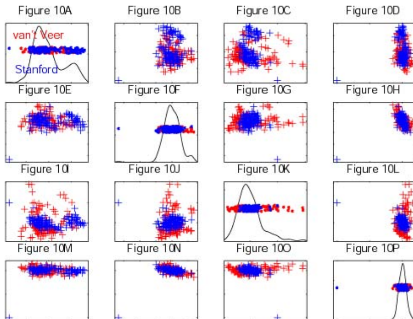
Figure 10: Scatterplot matrix of PCA projections, for the adjusted Stanford - van't Veer data. Overlap of the color groups shows an effective adjustment.
