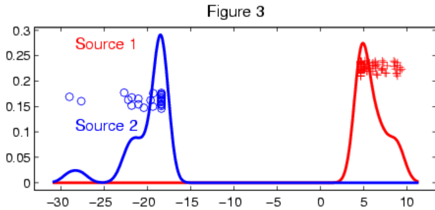
Figure 3: Projection of data from Figure 5, onto the normal vector of the SVM separating plane. Shows good separation of subpopulations, but data are piled up at margin.
