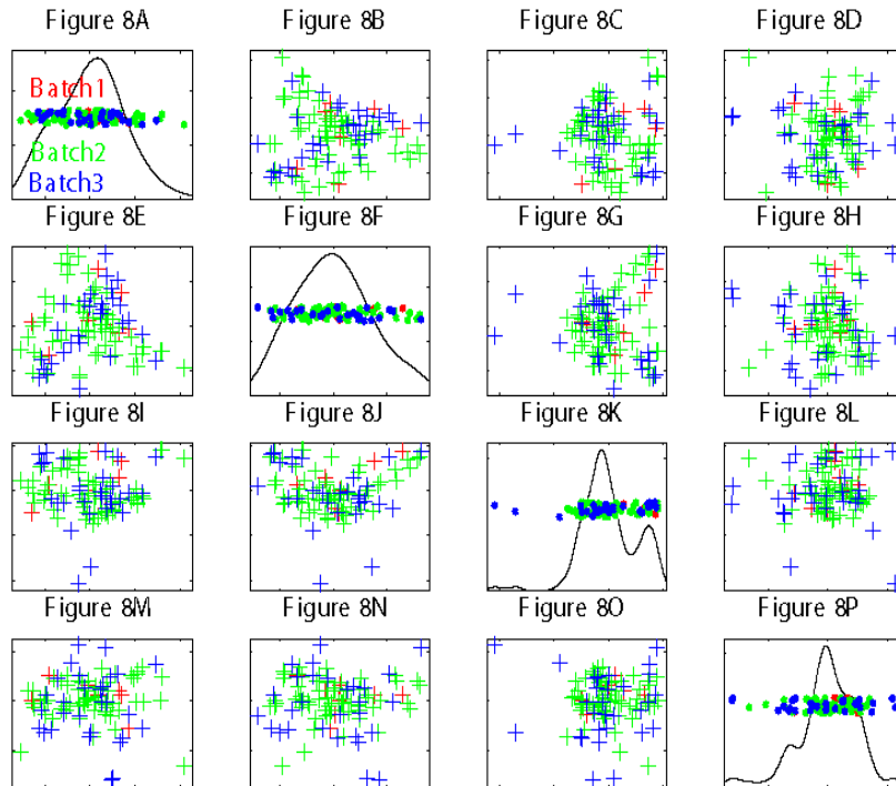
Figure 8: Scatterplot matrix of PCA projections, after DWD adjustment, of Stanford data. Random dispersion of colors again indicates adjustment was effective.
