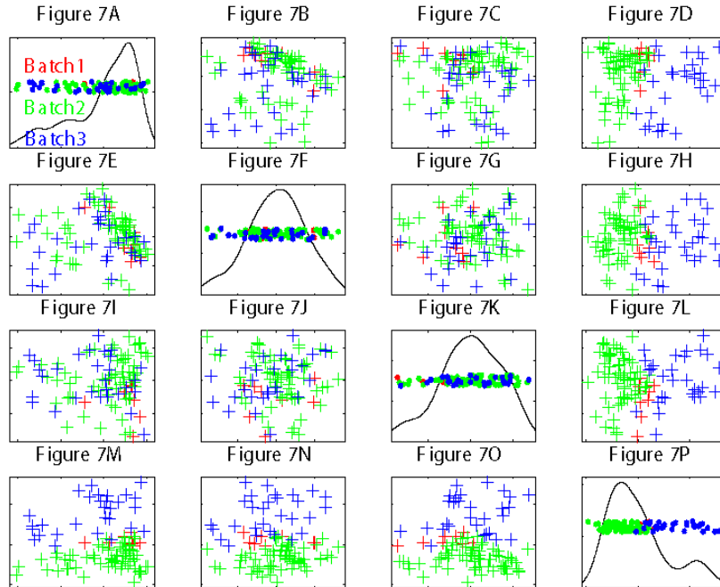
Figure 7: PCA projection scatterplot matrix of raw Stanford data, using batch colorings. Groupings of colors this time indicate serious batch effect problems, in a way that leaves conventional PC1 adjustment completely ineffective.
