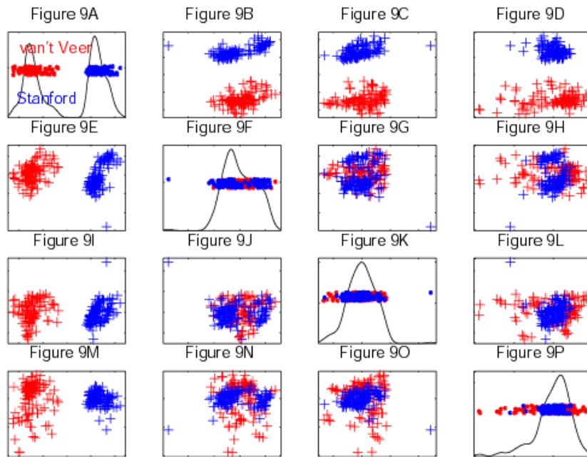
Figure 9: PCA projection scatterplot matrix of raw combined Stanford (blue) - van't Veer et al (red) data. Strong grouping by colors highlights the major differences between these platforms.
