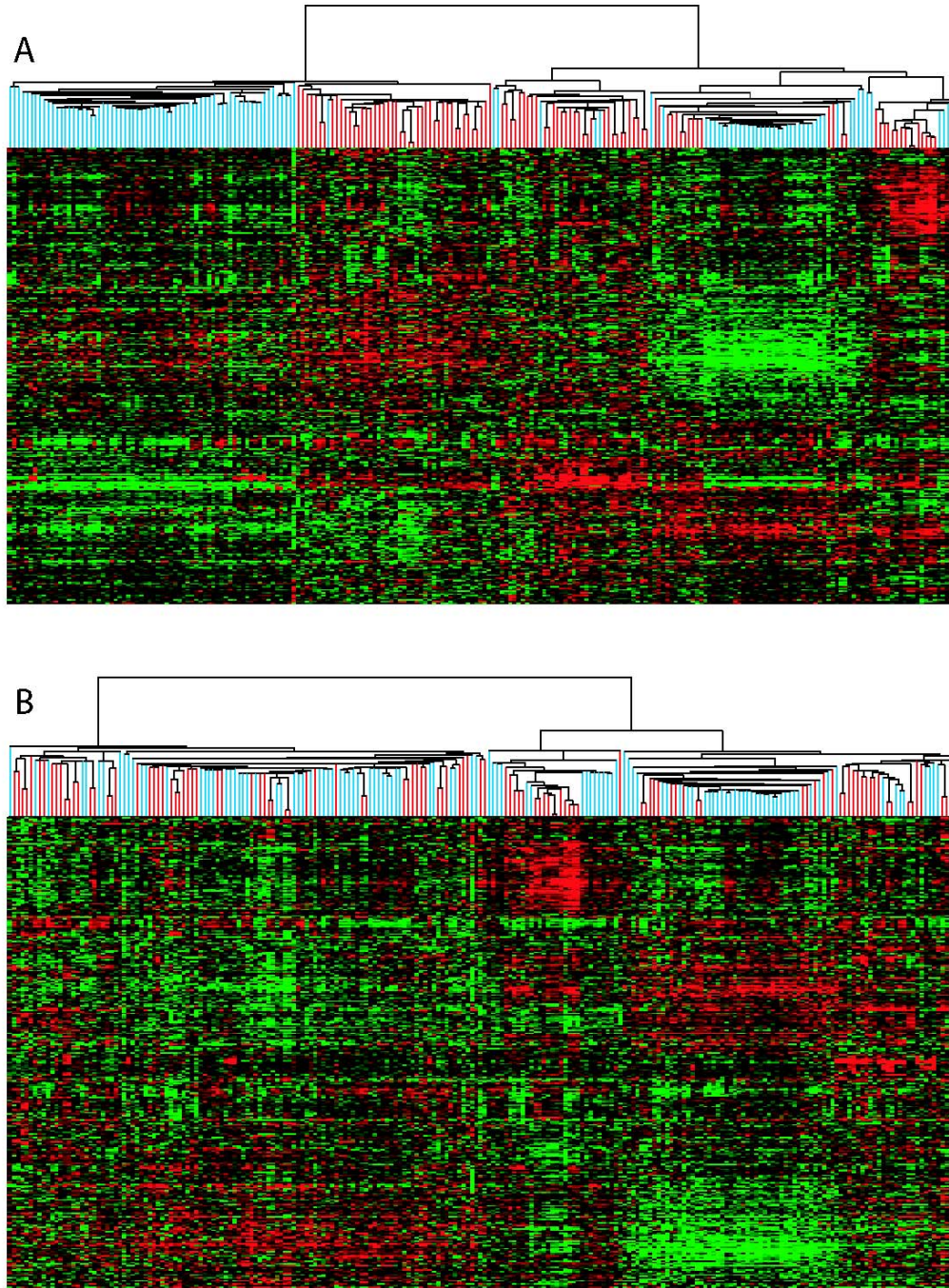
Figure 11: Hierarchical clustering analyses of unadjusted and adjusted data, with the van't Veer et al cases shown in red, and the Stanford cases blue. Figure 11A shows that simple median recentering, provides inadequate mixing across platforms, resulting in red-green gene patterns driven in part by batch effect. However, after the DWD platform adjustment resulting in Figure 11B, excellent mixing of the cases from the different platforms/groups was seen, resulting in red/green gene expression patterns of greater biological coherence.
