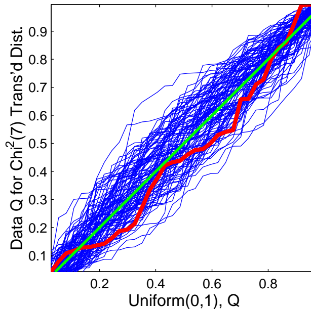
Unif. QQ for \alpha = 0.7 Power Trans.
