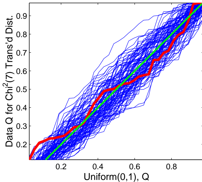
Unif. QQ for \alpha = 0.5 Power Trans.
