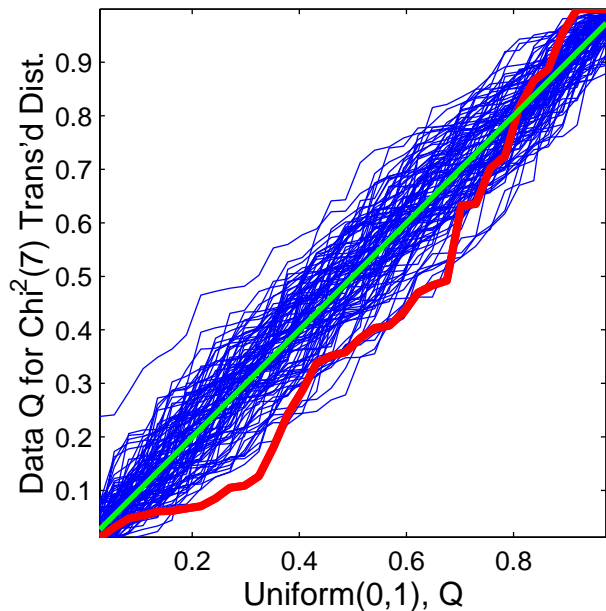
Unif. QQ for \alpha = 0.9 Power Trans.
