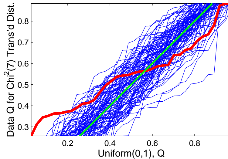
Unif. QQ for \alpha = 0.3 Power Trans.
