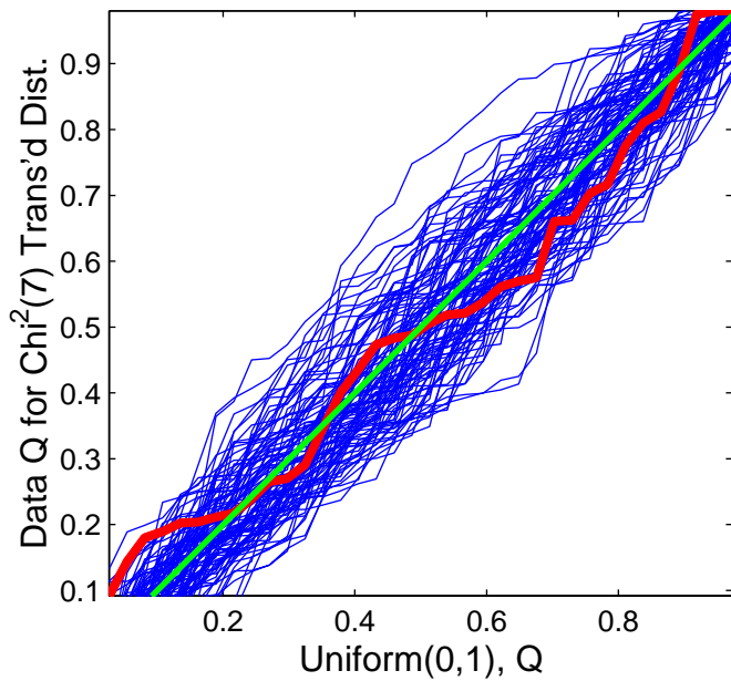
Unif. QQ for \alpha = 0.55 Power Trans.
