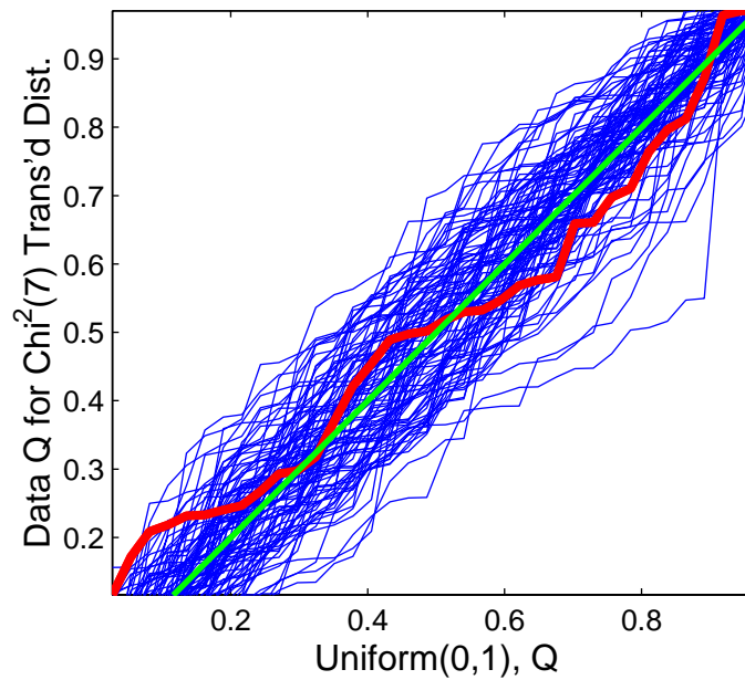
Unif. QQ for \alpha = 0.5 Power Trans.
