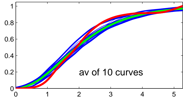
Dist to origin of data and transfd Gauss
