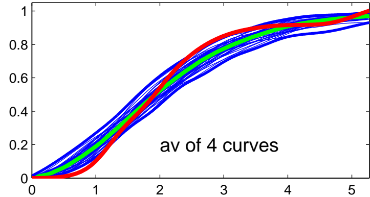
Dist to origin of data and transfd Gauss
