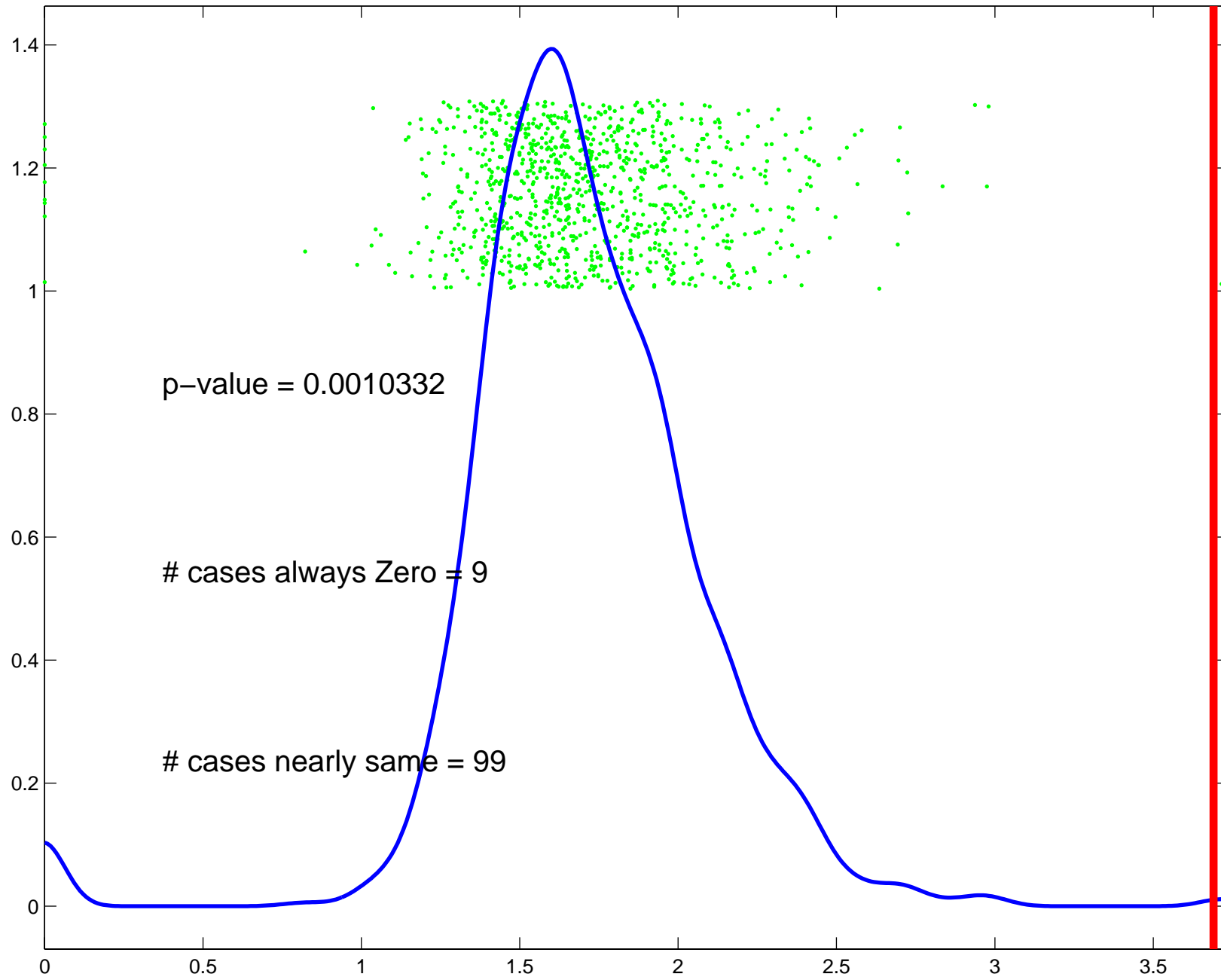
Abs Skew IC1 Gauss. test, max of r = 10 rep's
