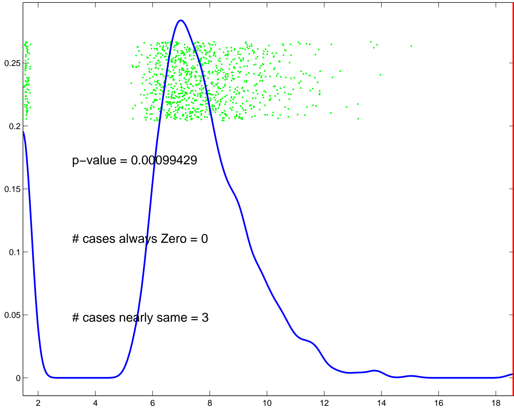
Kurtosis IC1 Gauss. test, max of r = 10 rep's
