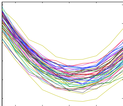
FIGURE 1A: Toy “raw data set” of curves. For illustration of concept of “understanding population structure”. The horizontal axis represents time, and the longitudinal variable of interest is on the vertical axis.
