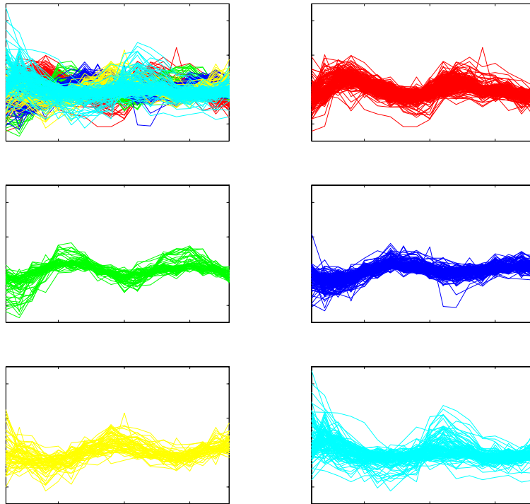
FIGURE 8: Raw time series view of the results of our classification. For each plot, time is on the horizontal, and relative gene expression level is on the vertical, axes. Show very clear grouping of genes into phase groups.
