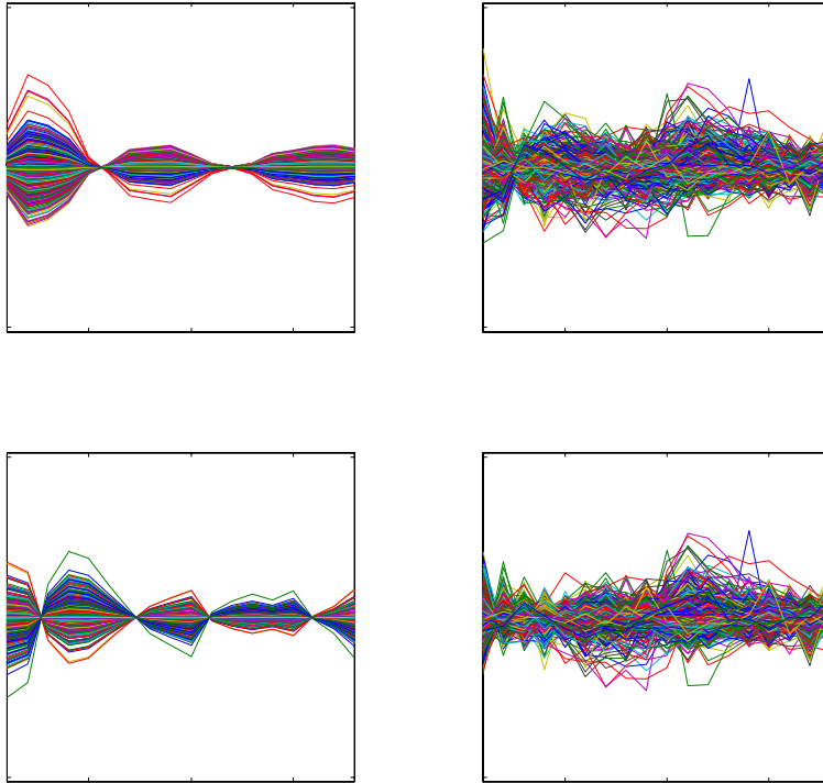
FIGURE 2B: PCA of gene expression time series from Figure 2B (with the same axes). Left panels are projection onto first (top) and second (bottom) PC directions (analogs of the bottom row of Figure 2B and the top row of Figure 2C). Right panels are corresponding residuals. Show nearly periodic structure, but not quite period 2.
