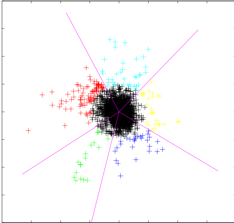
FIGURE 6: Projected scatterplot view of our gene classification, using the same data and axes as Figure 4. Black genes in the center are unclassified. Other colors represent the 5 classes. Suggests clear groupings of cell cycle phases.
