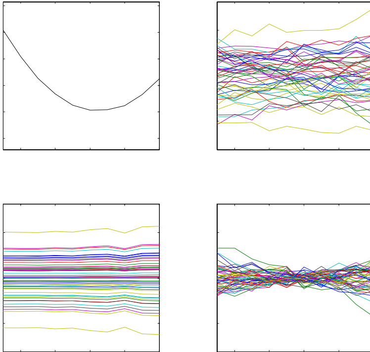
FIGURE 1B: Decomposition of variation in toy data set from Figure 1a (using the same axes). Upper left shows the mean. Upper right is residuals from mean. Lower left is projections of the mean residuals in the PC1 direction. Lower right is further residuals from PC1 projections.
