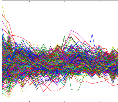
FIGURE 2A: Raw cell cycle gene expression time series. Horizontal axis represents time (over 2 cell cycles), vertical axis is relative level of gene expression. Each curve shows how the expression of a gene evolves over time.
