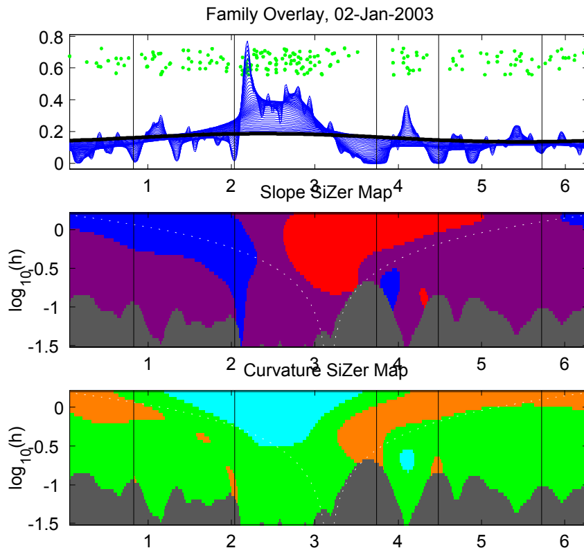
FIGURE 5: SiZer analysis of phases of top 200 most periodic genes, indicating clusters in the data that are statistically significant. The horizontal axis is phase (angles in radians), and the vertical axes are density (top), and bandwidth, i.e. scale or “level of resolution” (middle and bottom), Vertical lines are the boundaries that we found between the 5 cell phase classes.
