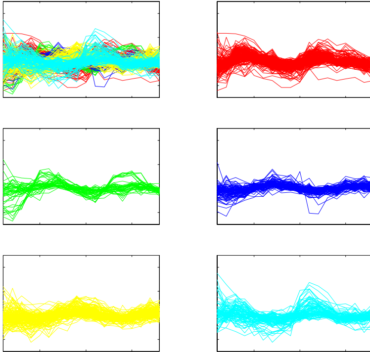
FIGURE 9: Raw time series view of the results of the Spellman, et al (1998) classification. Format is same as Figure 8. This gives a visual suggestion that our classification gave an improved identification of periodic genes.
