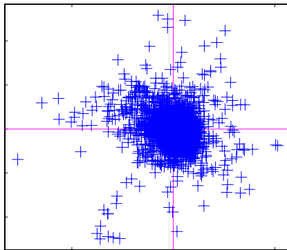
FIGURE 4: Scatterplot representation of the full data set, projected onto the subspace of the period 2 \sin and \cos function ( \cos on the horizontal, and \sin on the vertical, axes). Angle from the positive x -axis represents phase. Suggests that several phases are dominant.
