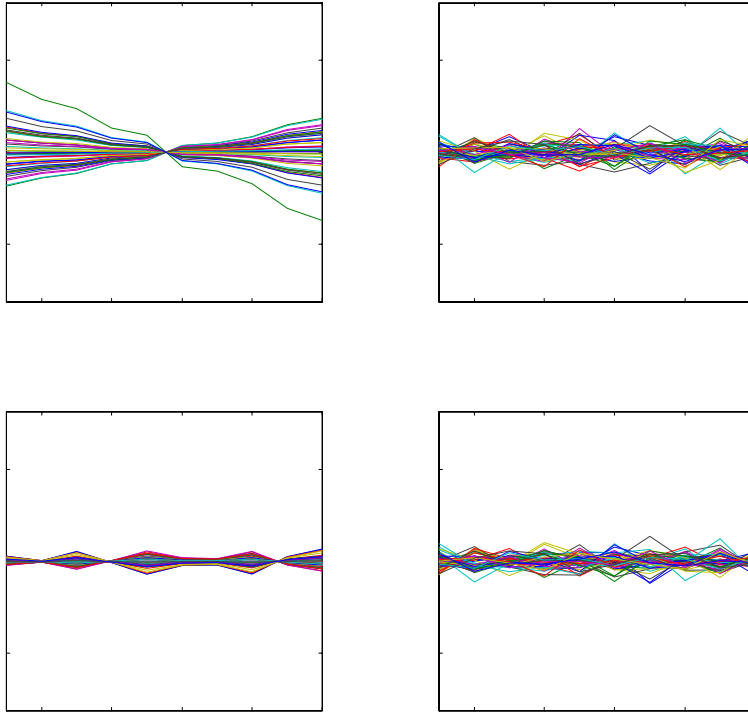
FIGURE 1c: Further visual decomposition of the variation of the data set from Figure 1a (using the same axes). Left side are projections in PC2 (upper) and PC3 (lower) directions. Right side are respective further residuals (starting from the lower right of Figure 1b).
