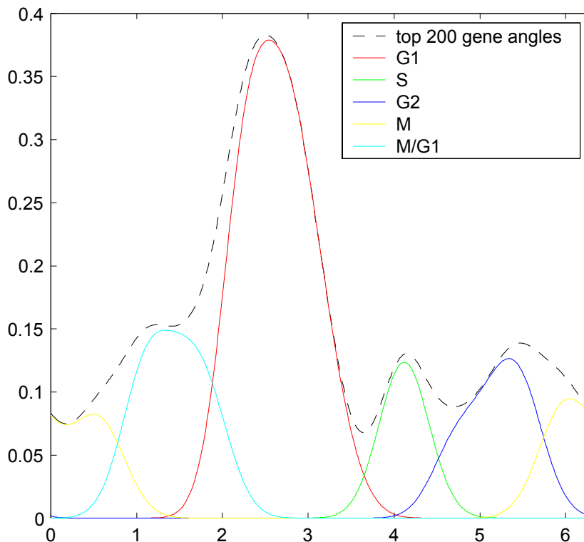
FIGURE 7: Smoothed histograms of populations of class phases. Phase (angle in radians) is on the horizontal, and density on the vertical, axes. Labels match class colors to named phases of cell cycle. Again suggests clear separation of periodic genes according to part of the cell cycle.
