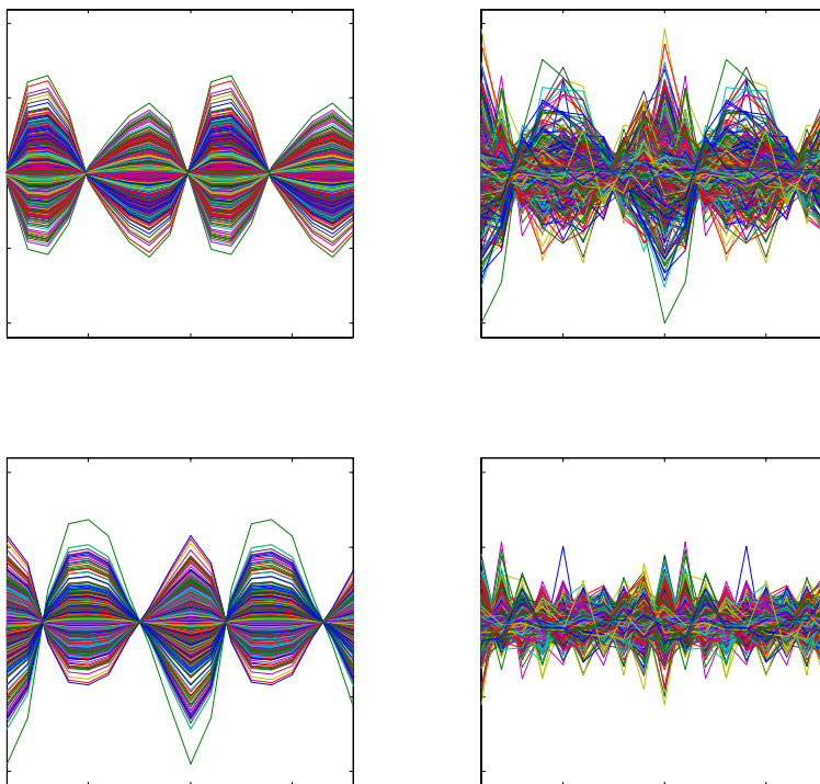
FIGURE 3B: PCA of frequency 2 projected cell cycle data (from Figure 3a, using the same axes), where the subplots are direct analogs of Figure 2b. PC projections on left, residuals on right. PC1 on top, PC2 on bottom. The two dominant directions are similar to the period 2 sin and cos functions, suggesting strong period 2 components.
