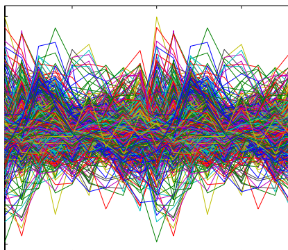
FIGURE 3A: Cell cycle time series (from Figure 2a, with the same axes), projected onto the subspace of frequency 2 harmonics. This is the “even periodic components” of the data from Figure 2a (note the left half is a replication of the right half).
