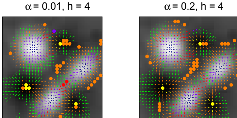
FIGURE 7: Gradient and Curvature version of S^3 , for simulated “Peaks and Valleys” example, using (a) \alpha = 0.01 (b) \alpha = 0.2 .
