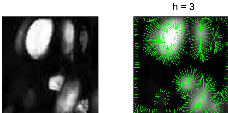
FIGURE 12: For the confocal data, (a) raw image, can structure on lower left be distinguished from back ground noise? (b) Streamline S^3 , shows structure on lower left is statistically significant.
