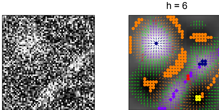
FIGURE 8: For simulated Peaks and Valleys example, with high noise \sigma = 0.4 , (a) Raw data, (b) Gradient and Curvature version of S^3 .
