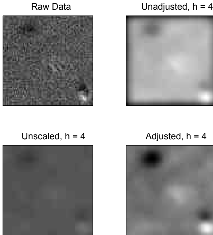
FIGURE 5: Image showing electrical activity. This illustrates boundary effects, and scaling issues.
