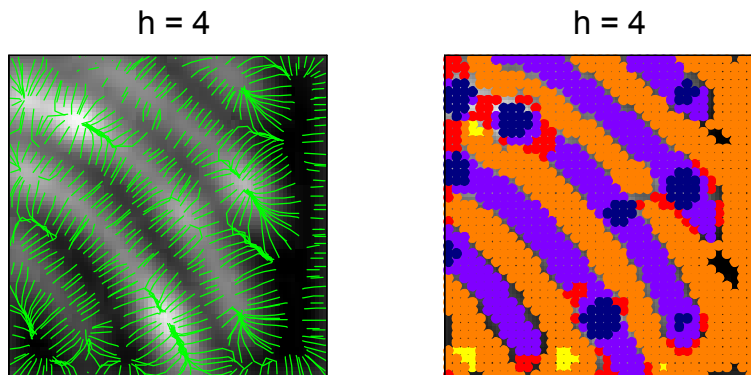
FIGURE 4: Streamline (a) and Curvature (b) based S^3 overlaid on a single smooth of the same subimage of the Gamma Camera Data. Streamlines in (a) gradient direction where significant. Dot colors in (b) indicate type of statistically significant curvature.
