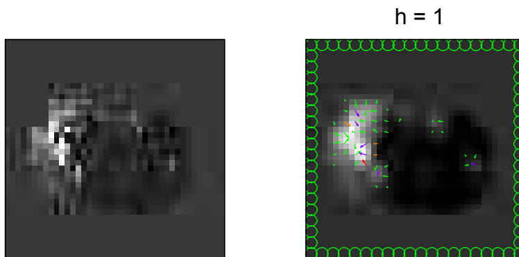
FIGURE 11: For the MRI perfusion data, (a) Raw data, (b) Gradient and curvature version of S^3 .
