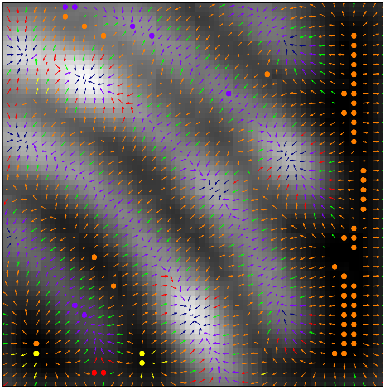
FIGURE 6: For the Gamma Camera Data, the combined gradient and curvature version of S^3 .
