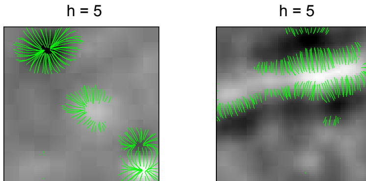
FIGURE 10: Streamline version of S^3 , (a) for “hot spot” part of Brain Activity data, (b) for “blood vessel” part of Brain Activity data.
