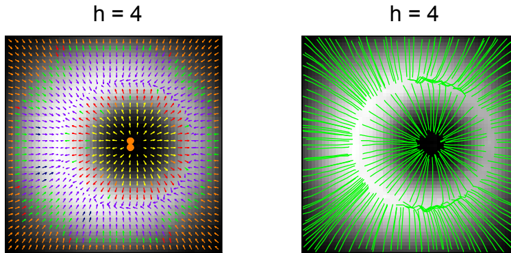
FIGURE 9: For simulated Volcano example, (a) Gradient and Curvature version of S^3 , (b) Streamline version of S^3 .
