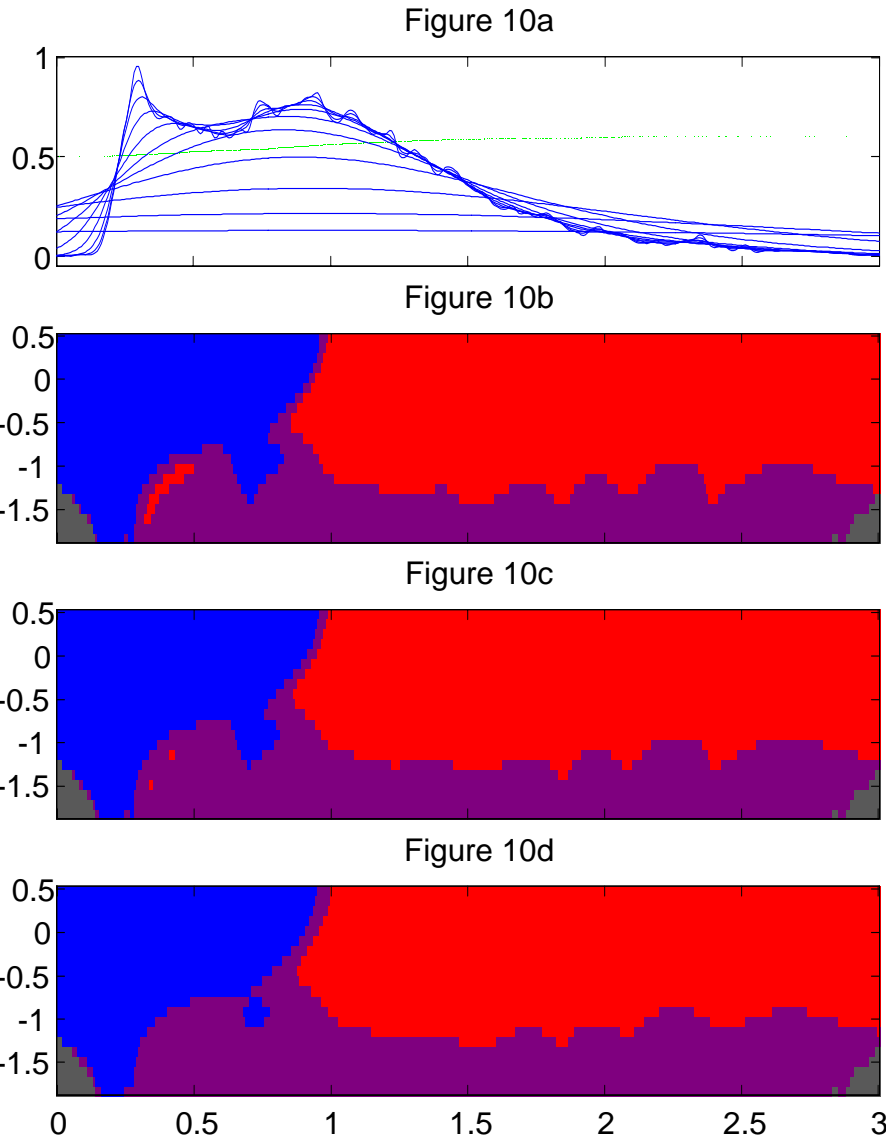
FIGURE 10: Full range of SiZer analyses of the British Family Incomes data. Figures 10a, b, c and d show family of smoothed curves, conventional, row-wise and global SiZer versions, respectively.
