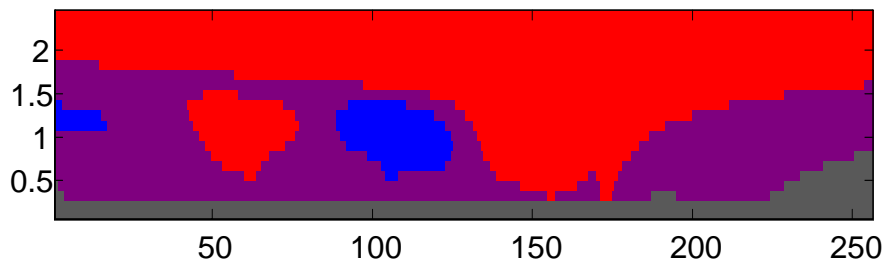
FIGURE 12: Full range of SiZer analyses of a flow cytometry data set. Figures 11a, b, c and d show family of smoothed curves, conventional, row-wise and global SiZer versions, respectively.
