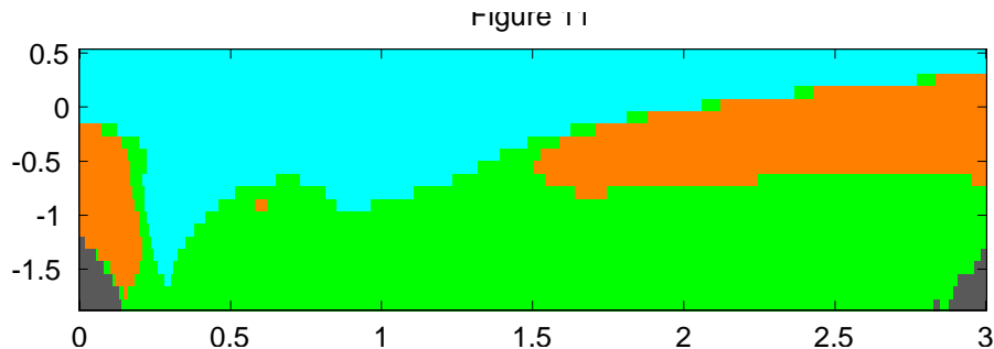
FIGURE 11: Global curvature SiZer analysis of the British Family Incomes data. This finds the bimodality that is known to be an important feature of this data set.
